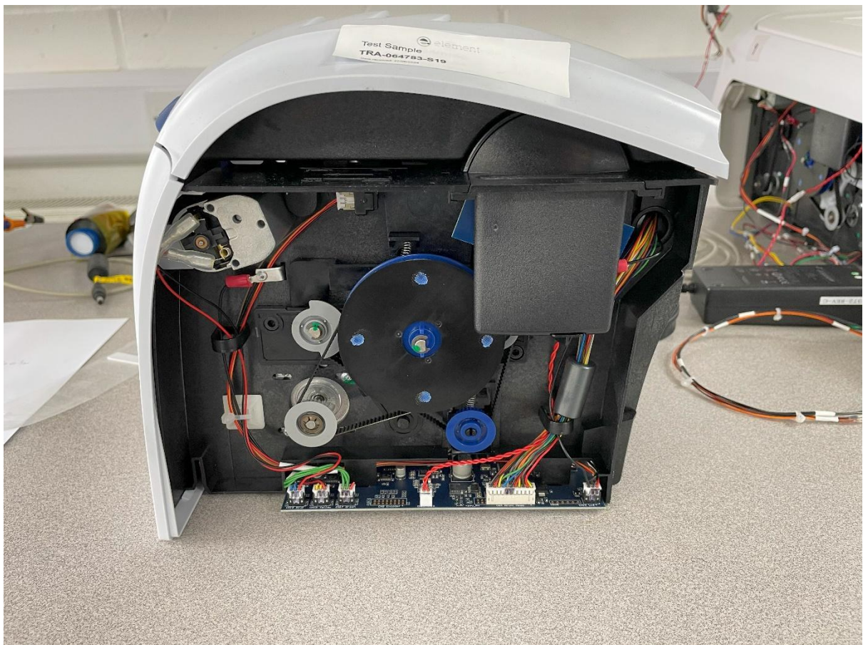
Figure 3: Internal right
