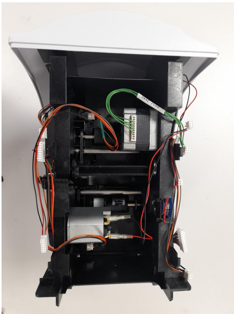
Figure 5: Internal underside (PCB removed)
