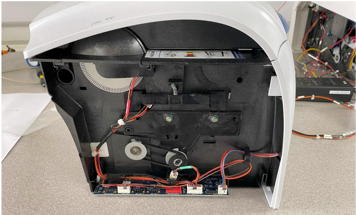
Figure 2: Internal left
