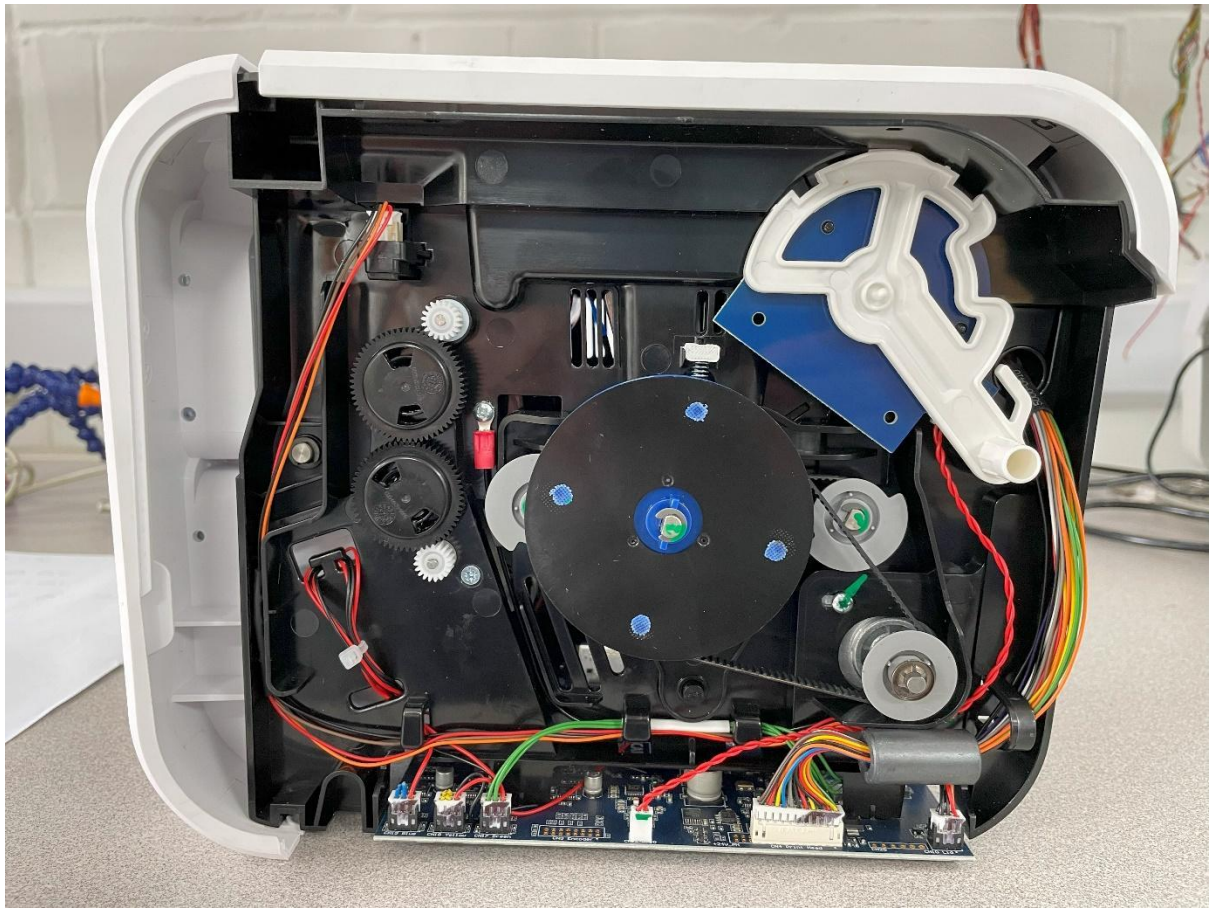
Figure 3: Internal right
