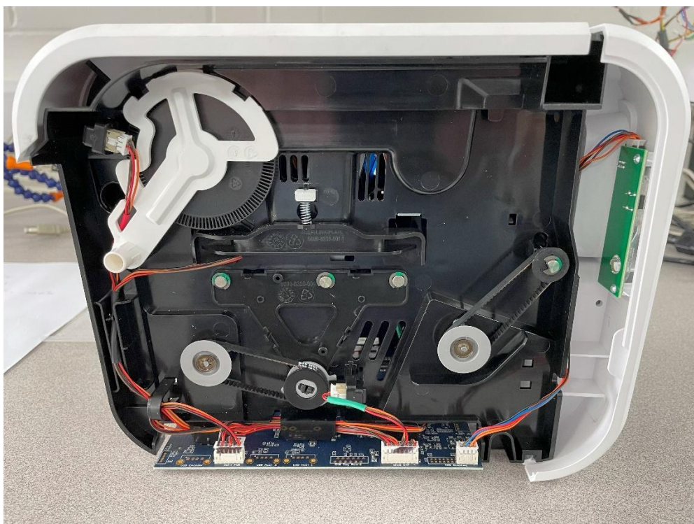
Figure 1: Internal left
