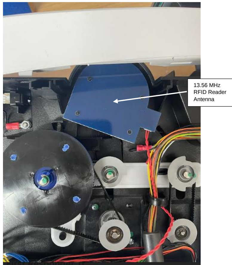
Figure 7: Close-Up view of view of RFID Antenna installed in product
