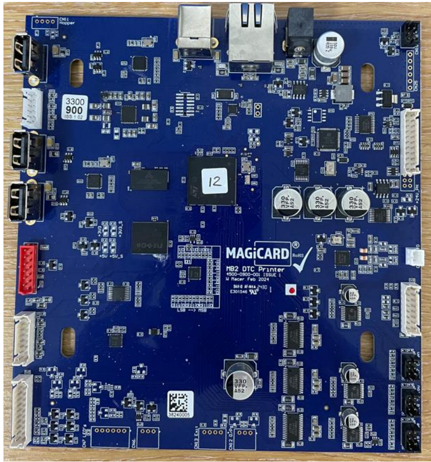
Figure 6: Top Side of PCB (PCB removed from product)
