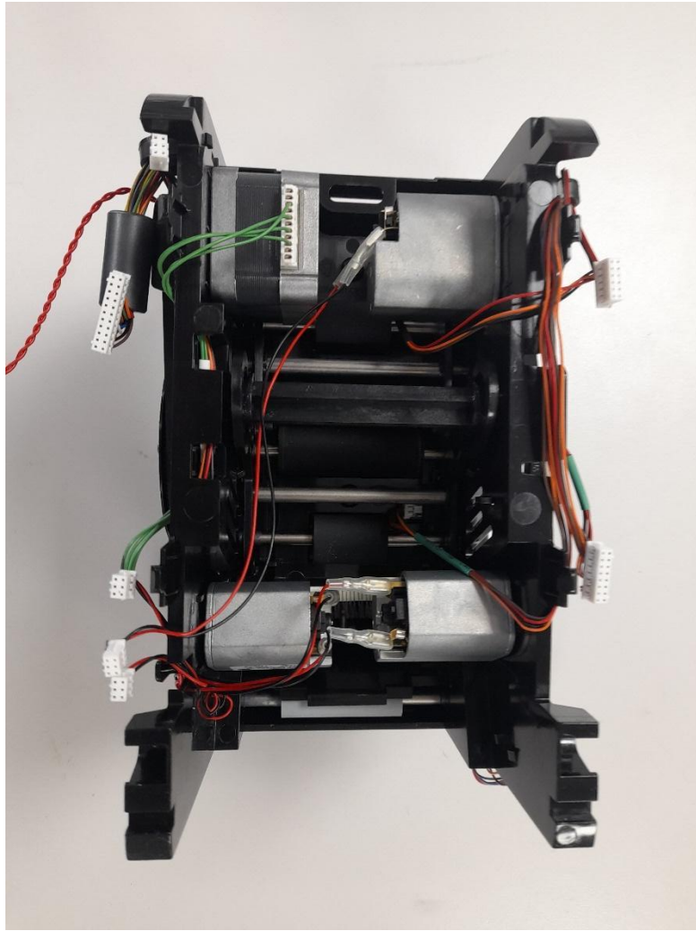
Figure 5: Internal bottom (PCB removed)
