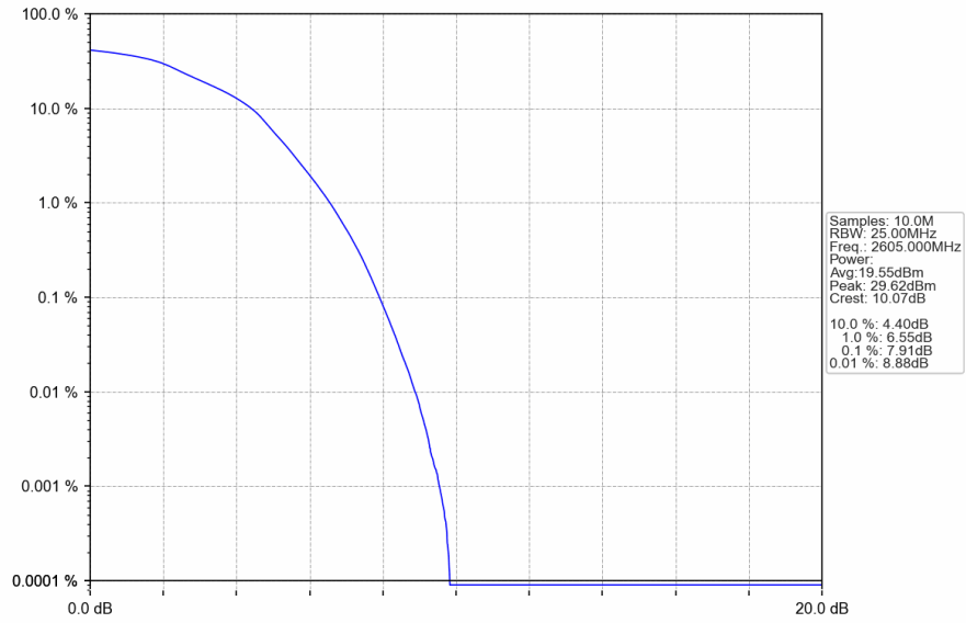
Band41_20MHz_16QAM_MCH_2605MHz_RB_100_0_NTNV
