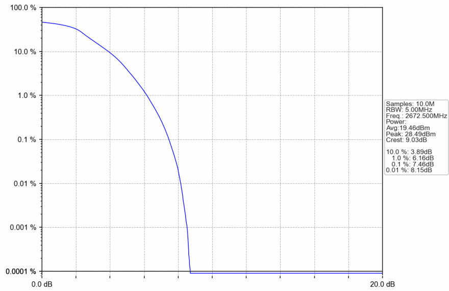
Band41_5MHz_QPSK_HCH_2672.5MHz_RB_25_0_NTNV
