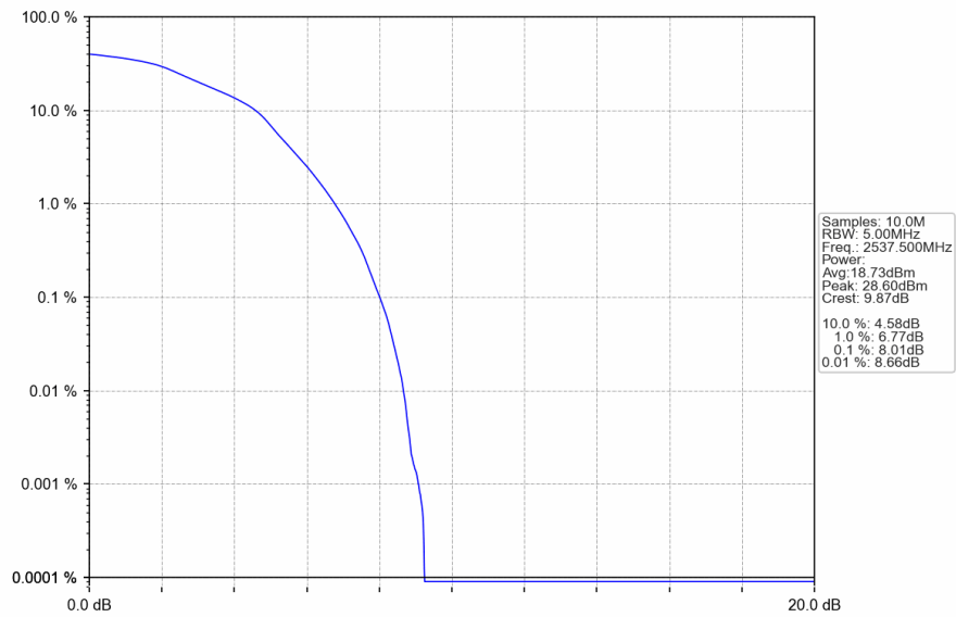
Band41_5MHz_16QAM_LCH_2537.5MHz_RB_25_0_NTNV
