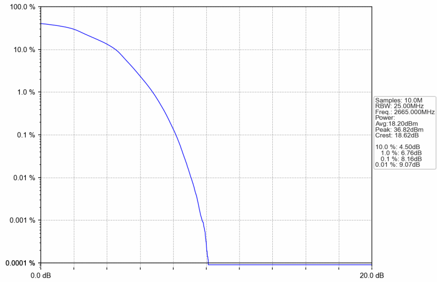
Band41_20MHz_16QAM_HCH_2665MHz_RB_100_0_NTNV
