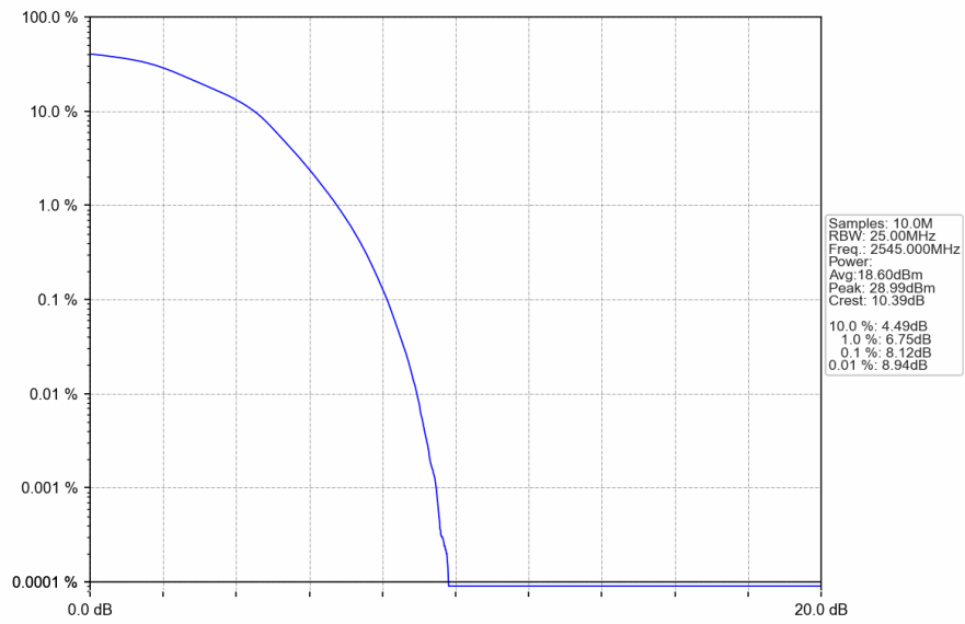
Band41_20MHz_16QAM_LCH_2545MHz_RB_100_0_NTNV
