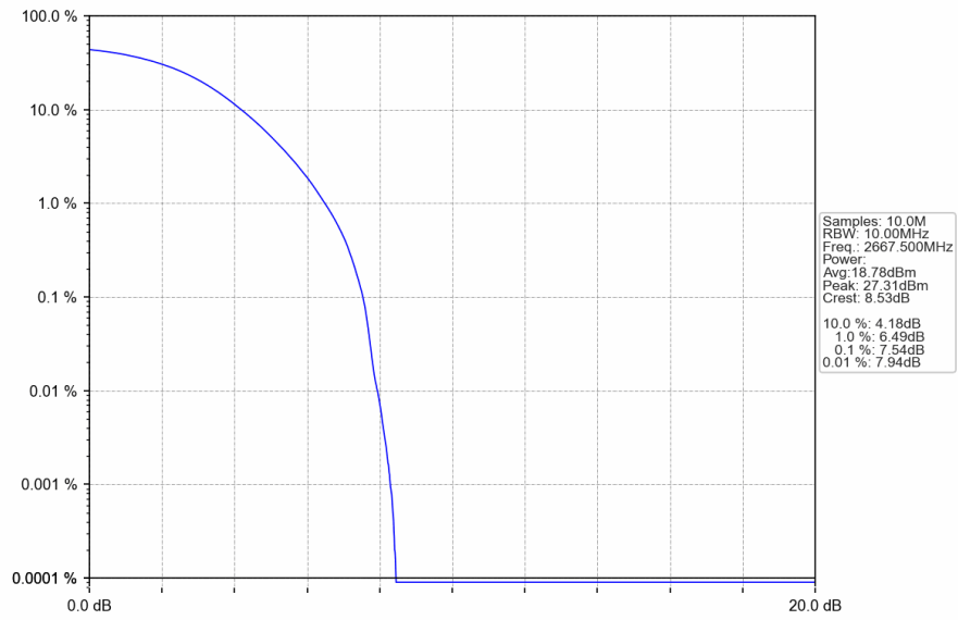
Band41_15MHz_QPSK_HCH_2667.5MHz_RB_75_0_NTNV
