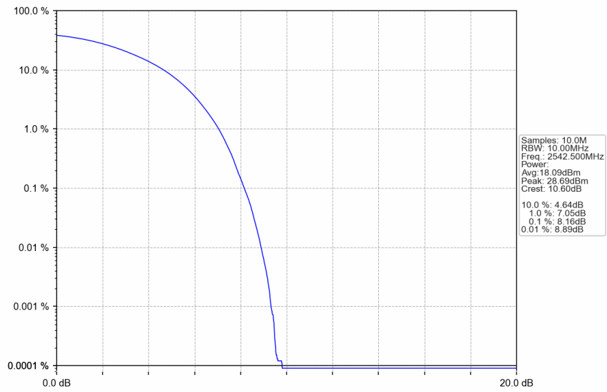
Band41_15MHz_16QAM_LCH_2542.5MHz_RB_75_0_NTNV
