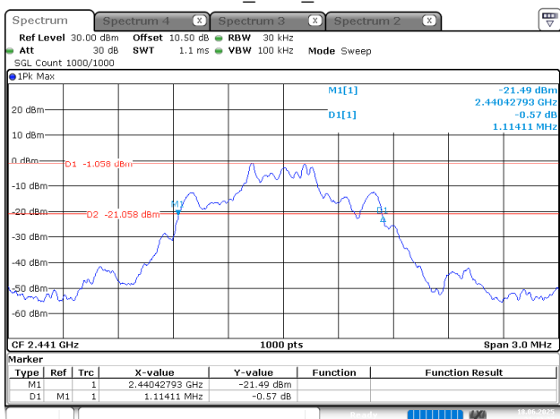
2EDR_DH1_Middle
