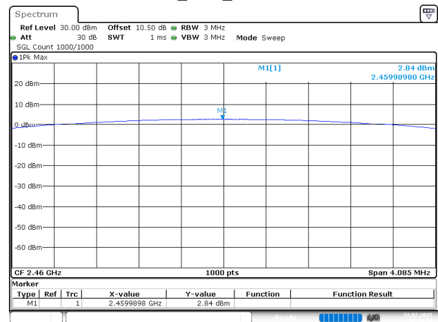
BDR_DH1_2460MHz
