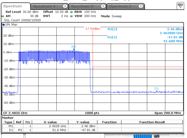
BDR_DH1_Hopping_Upper
