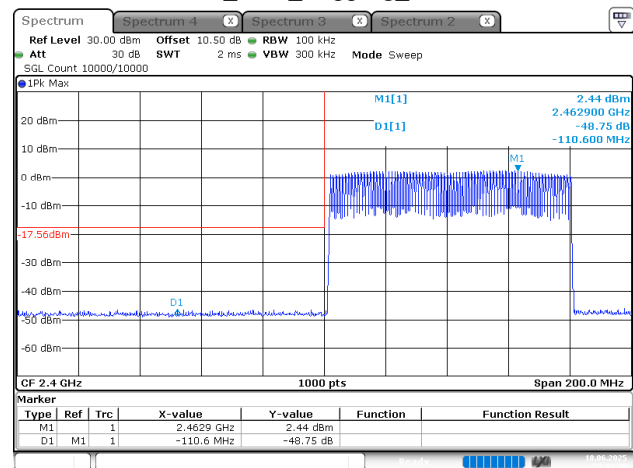
BDR_DH1_Hopping_Lower
