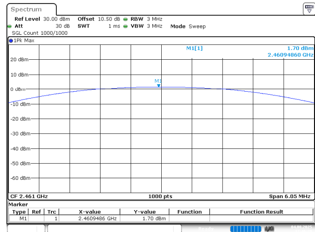
2EDR_DH1_2461MHz
