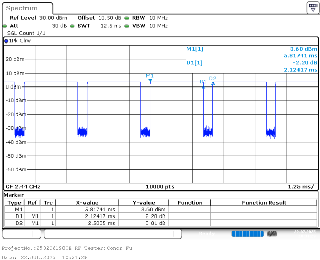
BLE_1M_Middle_Channel
