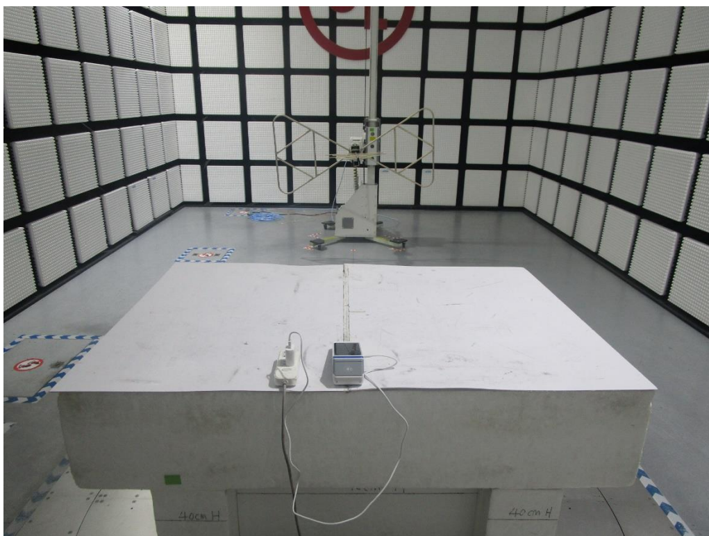
Radiated Band edge and Spurious Emission (Above 30 MHz and Below 1 GHz) (For NFC)
