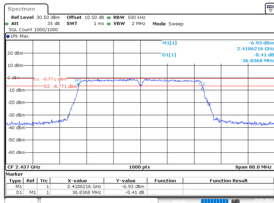
802.11n40_2437MHz
