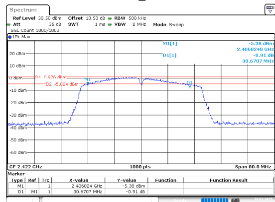
802.11n40_2422MHz
