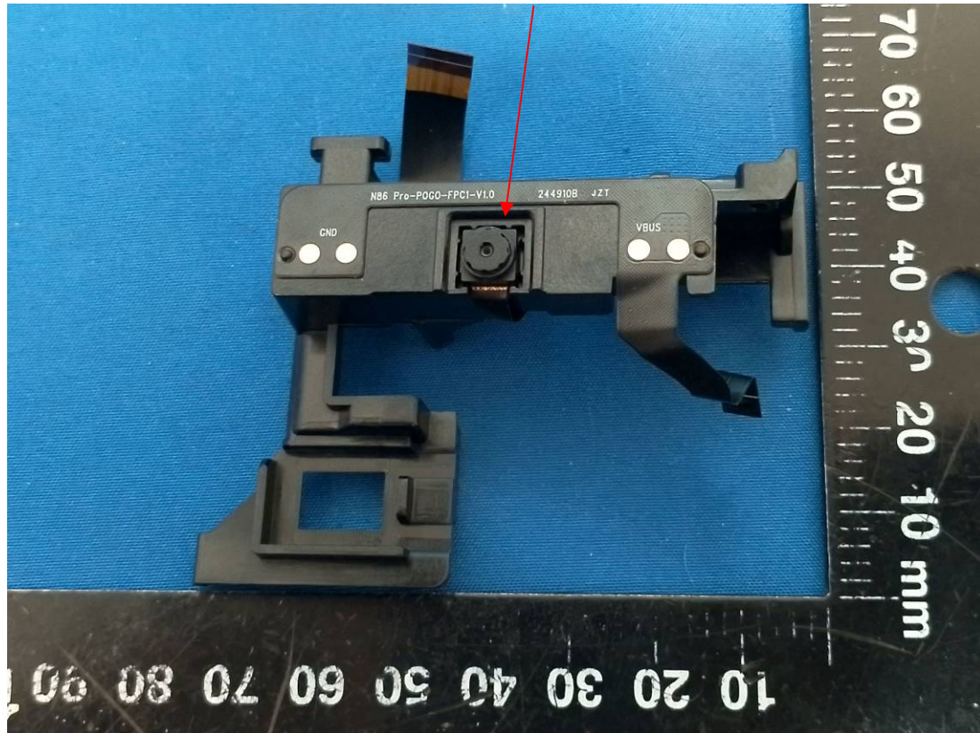
Back camera 2MP
