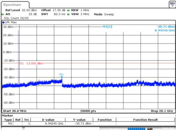
5MHz_High_QPSK_1@0(30MHz~20.1GHz)
