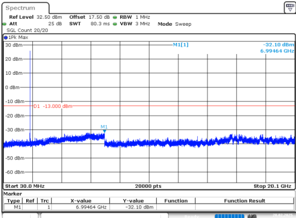
10MHz_Low_QPSK_1@0(30MHz~20.1GHz)
