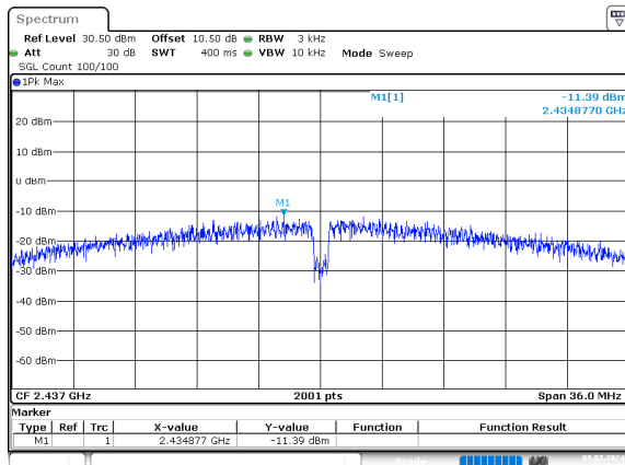
n40_2437MHz_Chain 0
