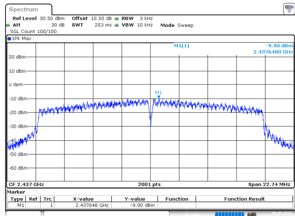
n20_2437MHz_Chain 0
