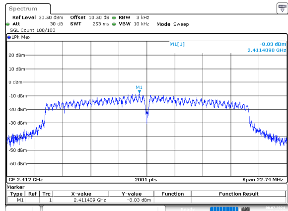
g_2412MHz_Chain 0
