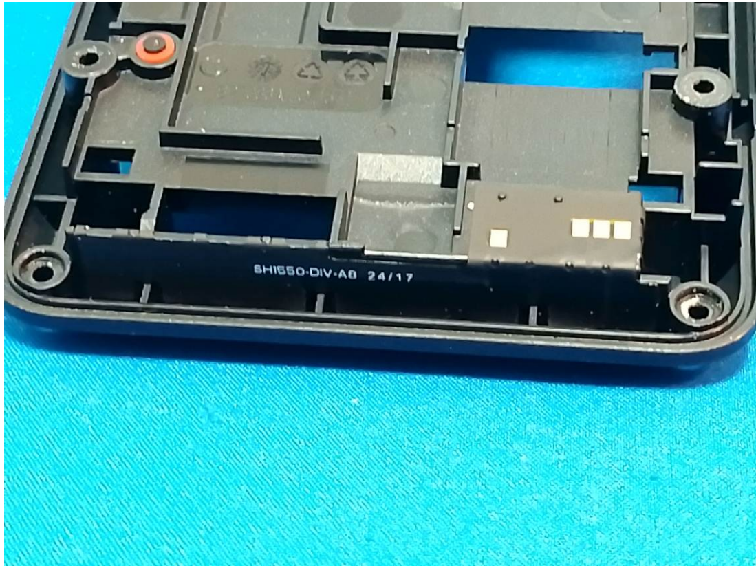
WWAN DIV Antenna(only for receive)
