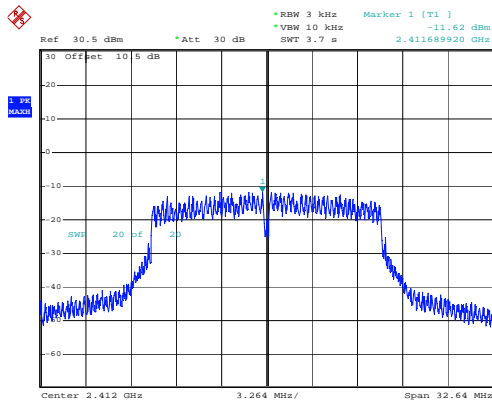
802.11g_2412MHz
