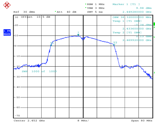
802.11n40_2452MHz
