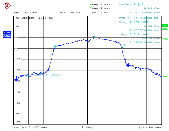
802.11n40_2437MHz
