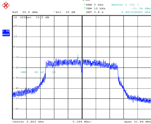
802.11g_2462MHz
