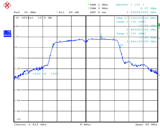
802.11n40_2422MHz
