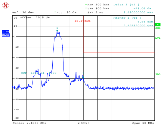
2EDR_2DH1_High
