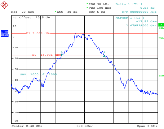
BDR_DH1_High
