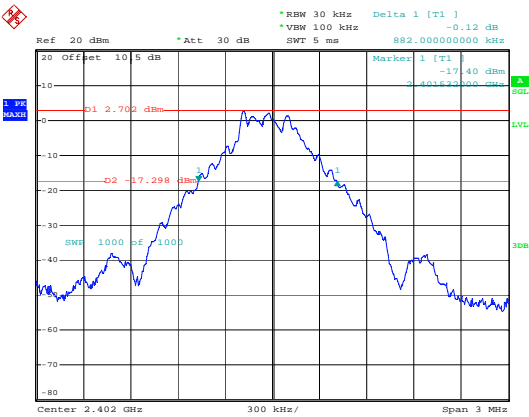
BDR_DH1_Low
