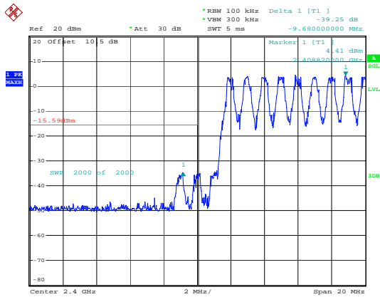
BDR_DH1_Hopping_Lower
