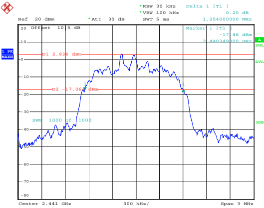
2EDR_2DH1_Middle
