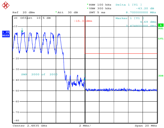
BDR_DH1_Hopping_Upper
