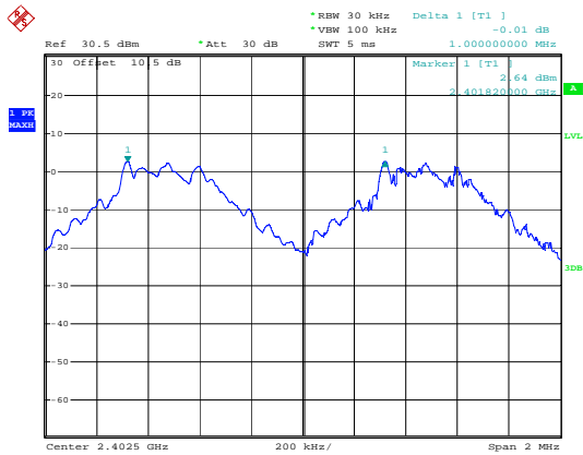
BDR_DH1_Low
