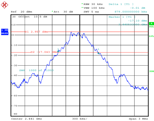
BDR_DH1_Middle
