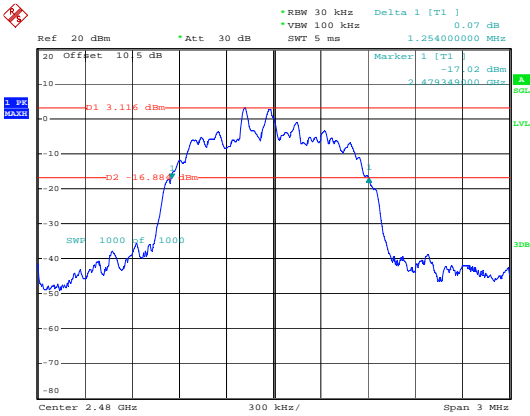
2EDR_2DH1_High
