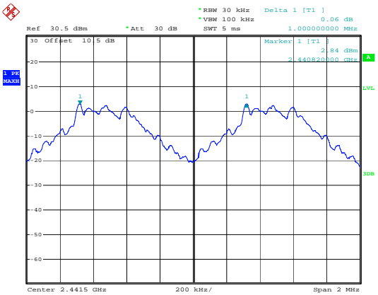
BDR_DH1_Middle
