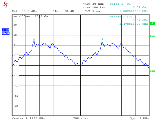
BDR_DH1_High
