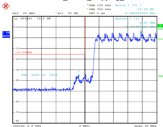
2EDR_2DH1_Hopping_Lower
