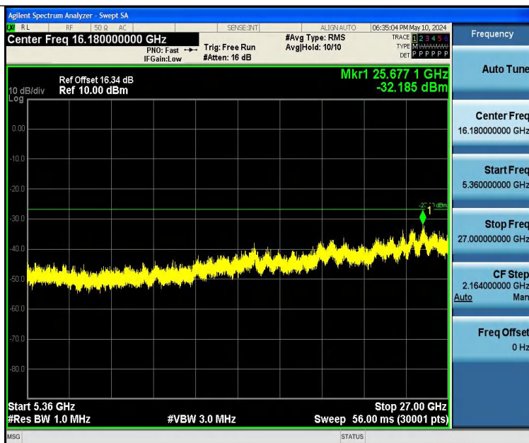
11N20SISO-Ant1-5200-5360~27000-PASS
