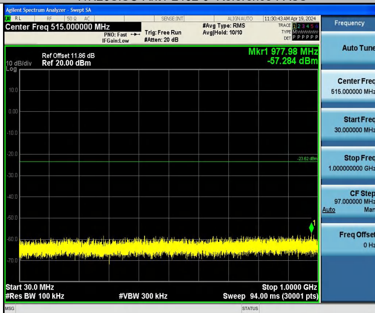
11N20SISO-Ant1-2462-30~1000-PASS
