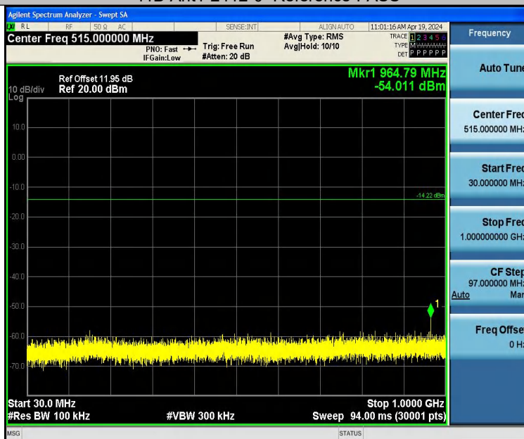
11B-Ant1-2412-30~1000-PASS
