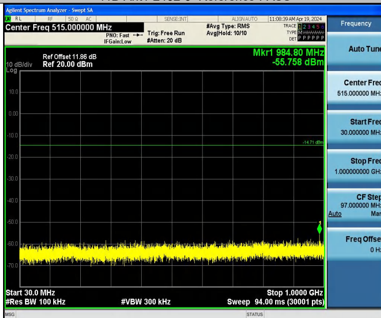
11B-Ant1-2462-30~1000-PASS
