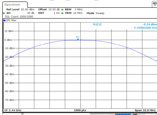
BLE_2M_Middle_Channel
