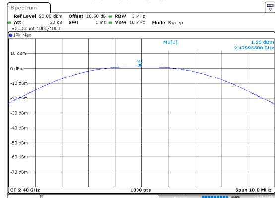
BLE_2M_High_Channel
