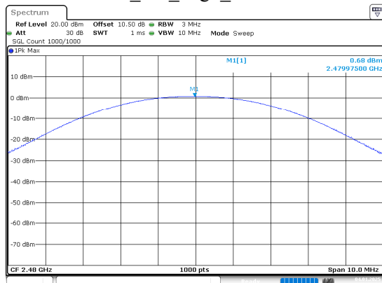
BLE_1M_High_Channel
