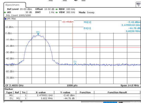
BLE_2M_High_Channel
