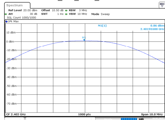
BLE_2M_Low_Channel
