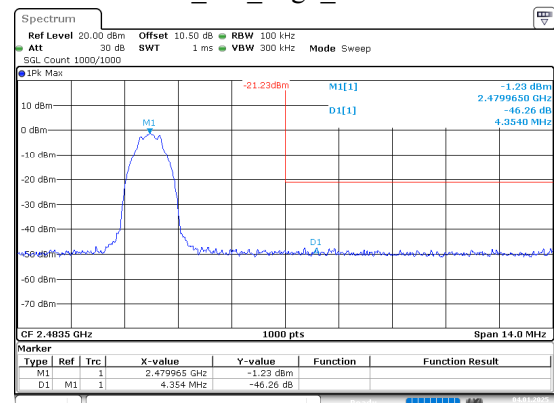
BLE_1M_High_Channel
