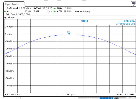
BLE_1M_Middle_Channel
