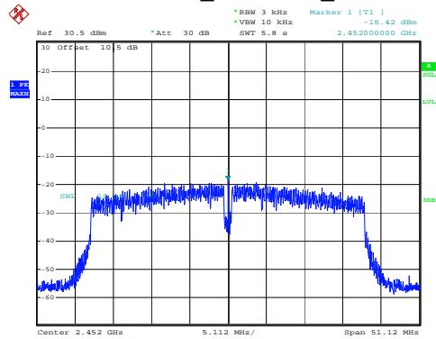
802.11n40_2452MHz_Chain 0
