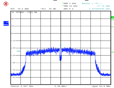
802.11n40_2437MHz_Chain 0
