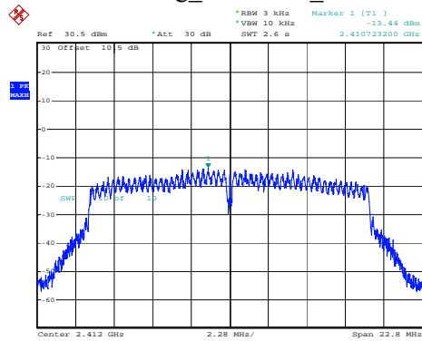
802.11g_2412MHz_Chain 0
