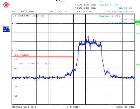
802.11g_2412MHz_Chain 1
