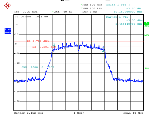
802.11g_2462MHz_Chain 0
