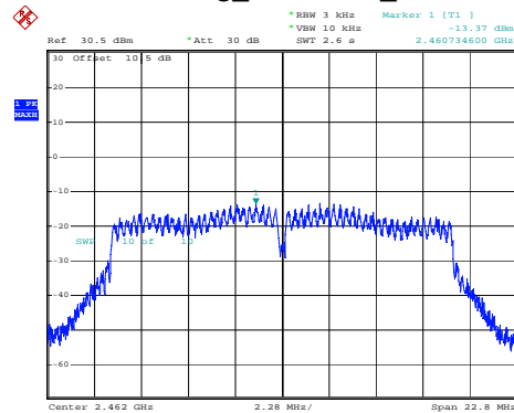
802.11g_2462MHz_Chain 1
