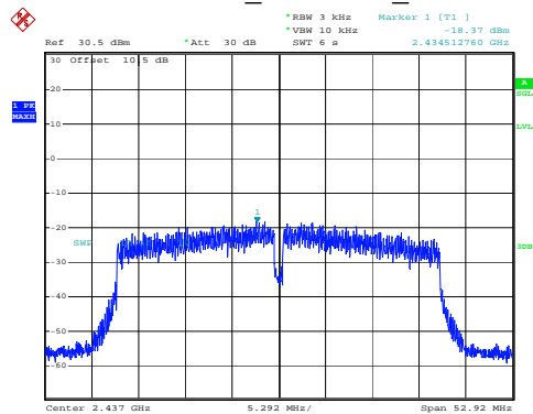
802.11n40_2437MHz_Chain 1
