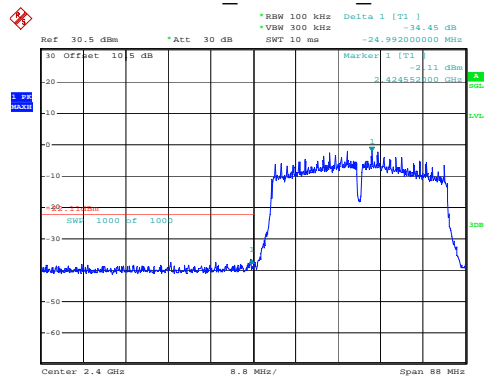
802.11n40_2422MHz_Chain 1
