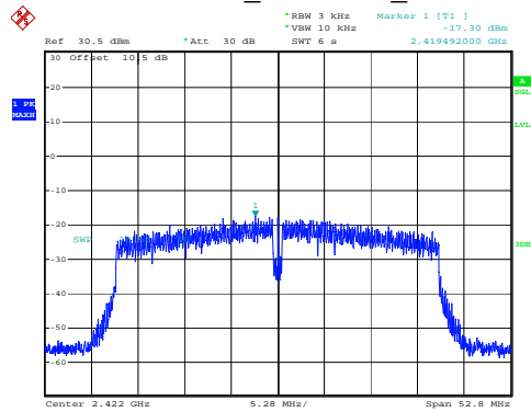
802.11n40_2422MHz_Chain 0
