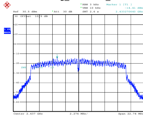
802.11g_2437MHz_Chain 0
