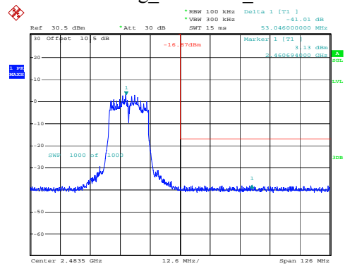
802.11g_2462MHz_Chain 1
