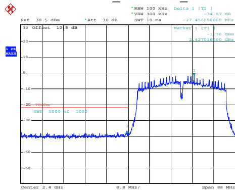
802.11n40_2422MHz_Chain 0
