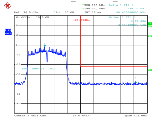
802.11n40_2452MHz_Chain 1
