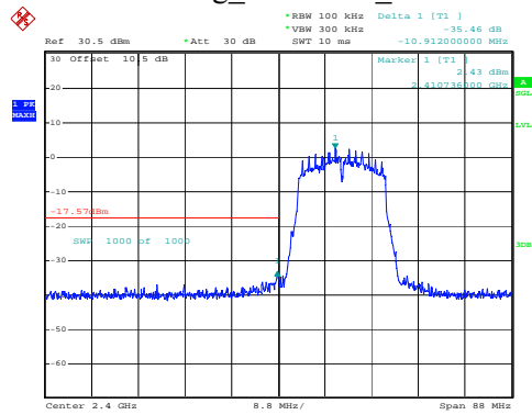
802.11g_2412MHz_Chain 0
