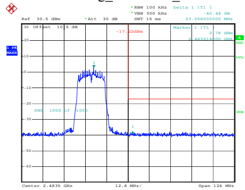
802.11g_2462MHz_Chain 0
