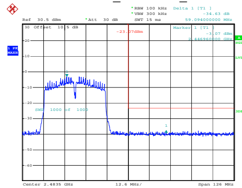
802.11n40_2452MHz_Chain 0
