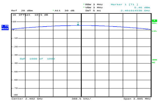
GFSK_Low
