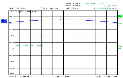
GFSK_High
