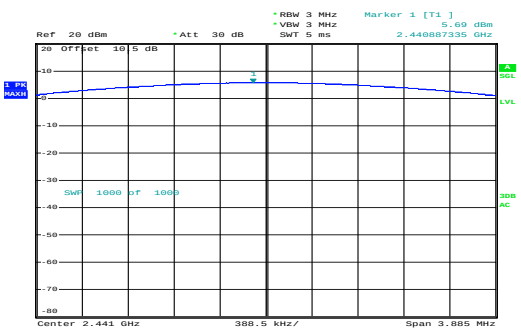
GFSK_Middle
