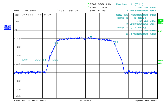
g_2462MHz_Chain 0
