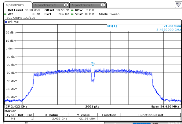
n40_2422MHz_Chain 0
