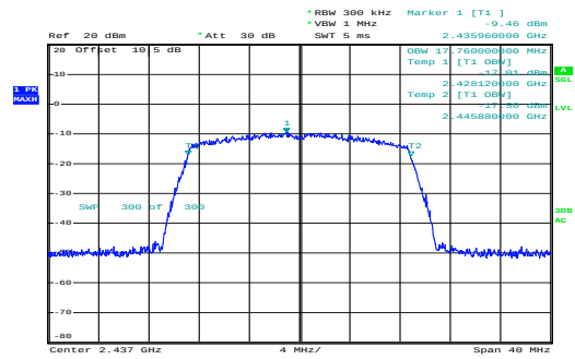
n20_2437MHz_Chain 0
