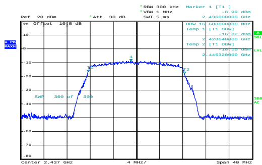
g_2437MHz_Chain 0 1
