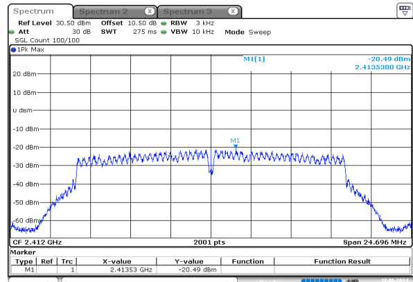
g_2412MHz_Chain 0
