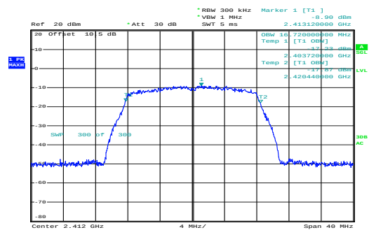
g_2412MHz_Chain 0
