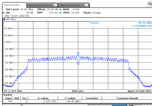
g_2437MHz_Chain 0
