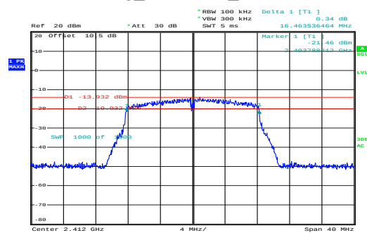
g_2412MHz_Chain 0
