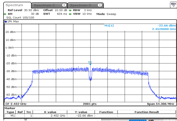
n40_2452MHz_Chain 0
