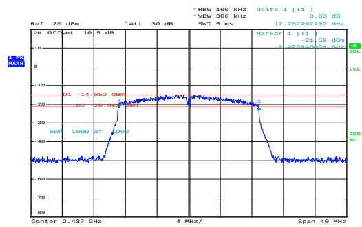
n20_2437MHz_Chain 0
