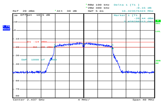
g_2437MHz_Chain 0
