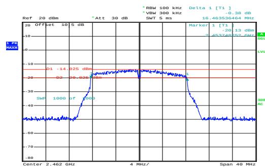
g_2462MHz_Chain 0
