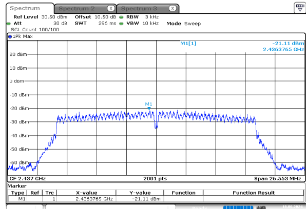
n20_2437MHz_Chain 0
