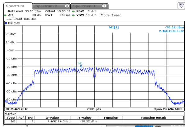
g_2462MHz_Chain 0
