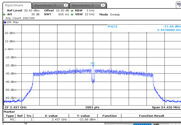
n40_2437MHz_Chain 0
