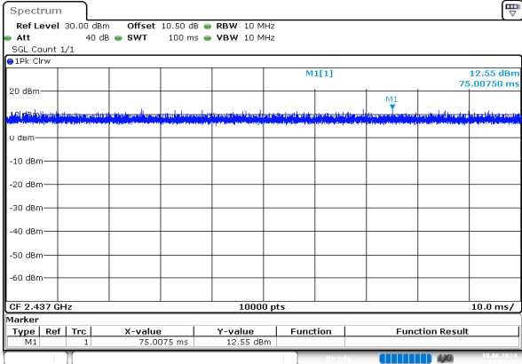
n20_2437MHz_Chain 0
