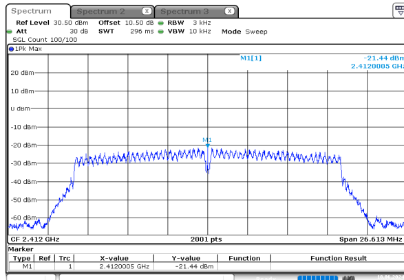
n20_2412MHz_Chain 0
