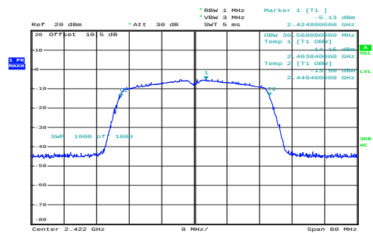
n40_2422MHz_Chain 0
