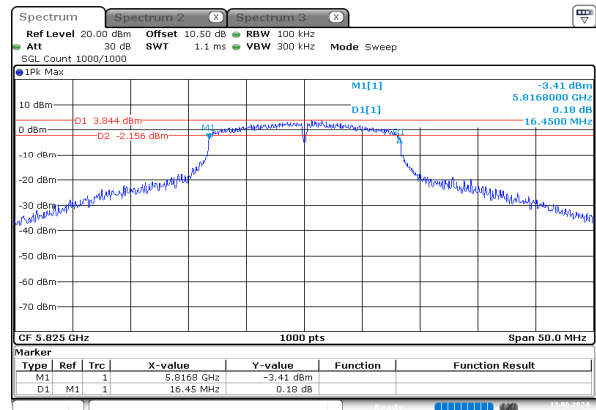
a_5825MHz_Chain 0
