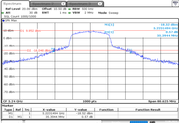
n20_5240MHz_Chain 0
