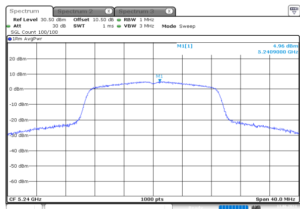
n20_5240MHz_Chain 0
