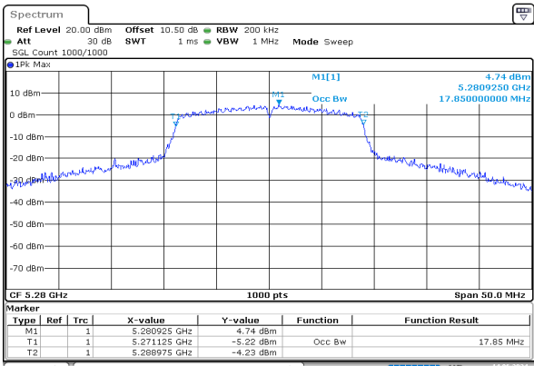
n20_5280MHz_Chain 0
