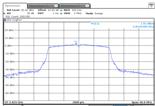
a_5825MHz_Chain 0
