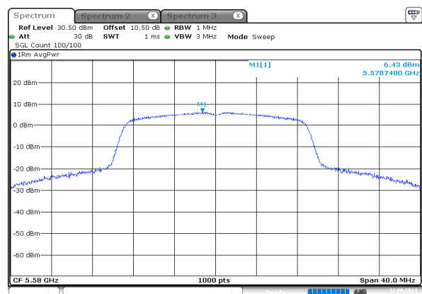
n20_5580MHz_Chain 0
