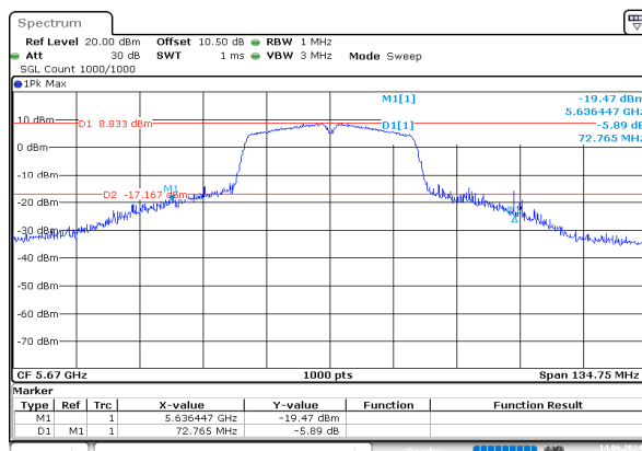
n40_5670MHz_Chain 0
