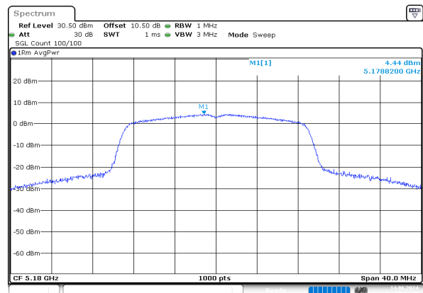
n20_5180MHz_Chain 0
