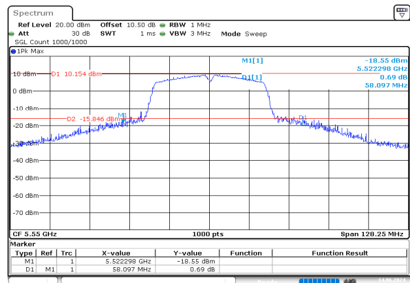
n40_5550MHz_Chain 0
