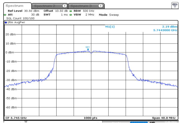
a_5745MHz_Chain 0
