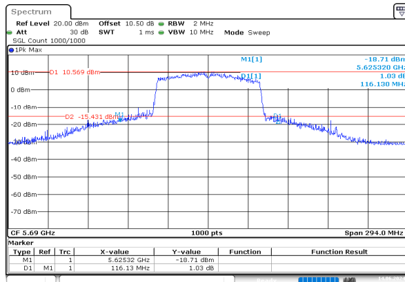
ac80_5690MHz_Chain 0
