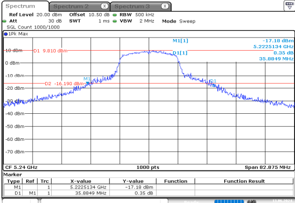
a_5240MHz_Chain 0
