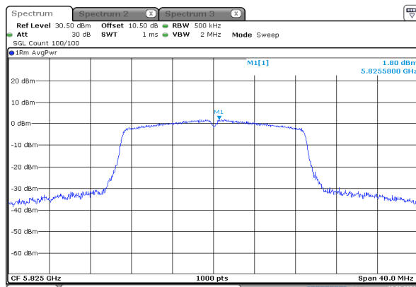
n20_5825MHz_Chain 0
