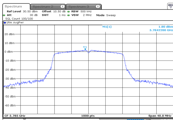
a_5785MHz_Chain 0
