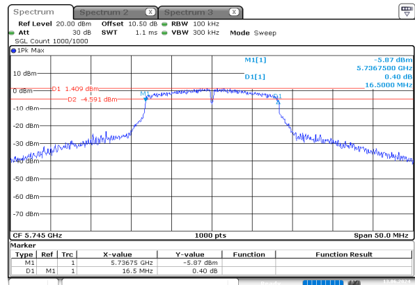
a_5745MHz_Chain 0
