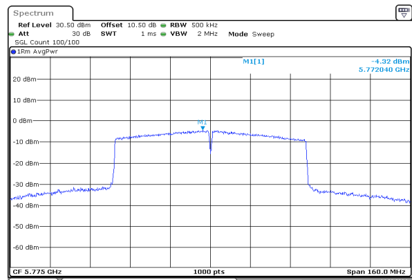
ac80_5775MHz_Chain 0
