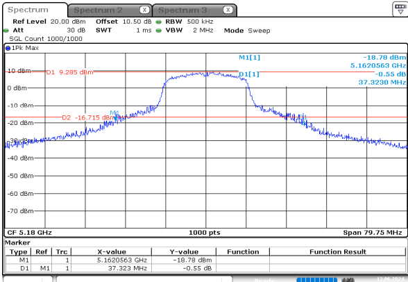
a_5180MHz_Chain 0
