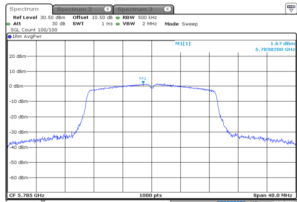
n20_5785MHz_Chain 0
