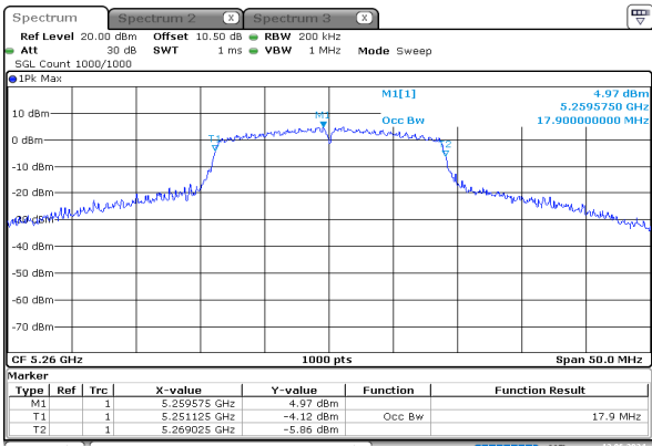
n20_5260MHz_Chain 0
