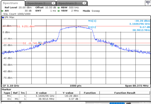
n20_5180MHz_Chain 0
