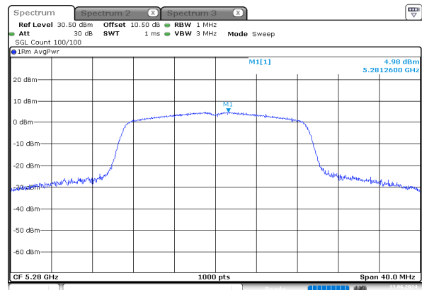
n20_5280MHz_Chain 0
