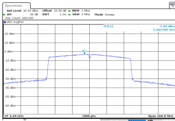
ac80_5690MHz_Chain 0
