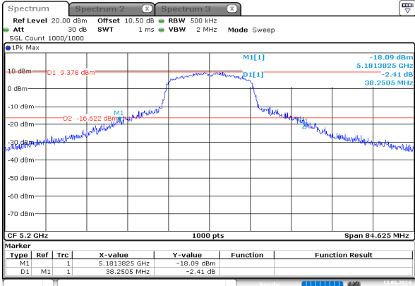
n20_5200MHz_Chain 0
