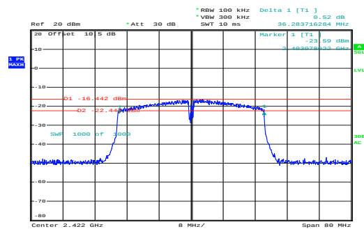
n40_2422MHz_Chain 0
