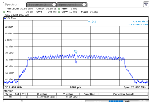
n20_2437MHz_Chain 0
