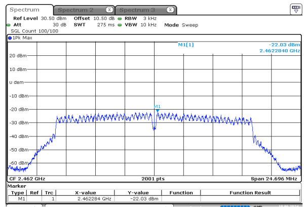
g_2462MHz_Chain 0
