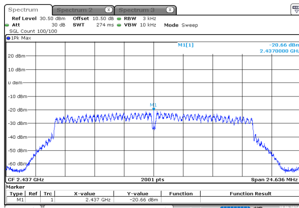
g_2437MHz_Chain 0
