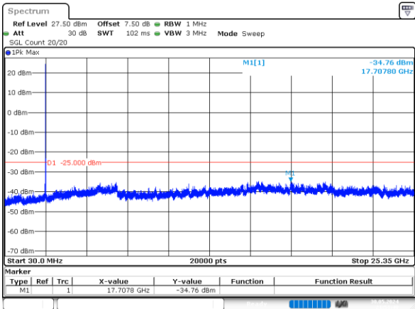
15MHz_Middle_QPSK_1@0 -34.76dBm
