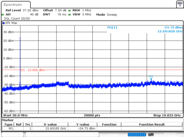
15MHz_High_QPSK_1@0 -24.73dBm
