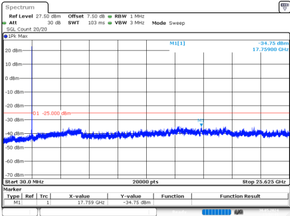
15MHz_High_QPSK_1@0 -34.75dBm
