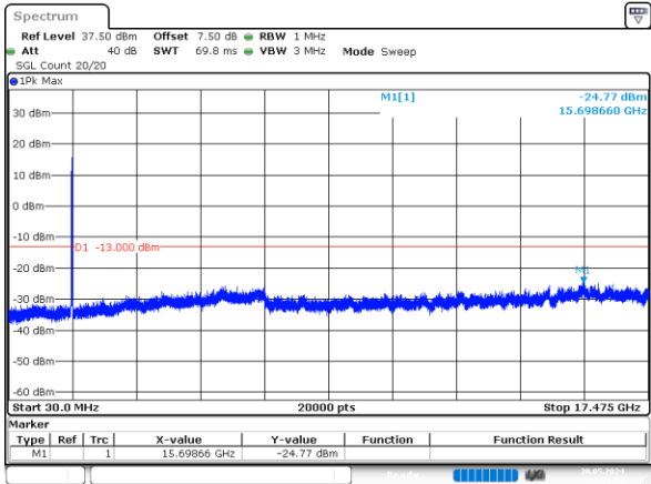
15MHz_High_QPSK_75@0 -24.77dBm
