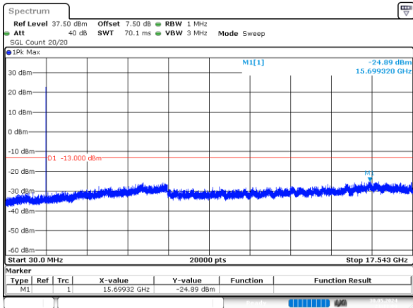
1.4MHz_High_QPSK_6@0 -24.89dBm
