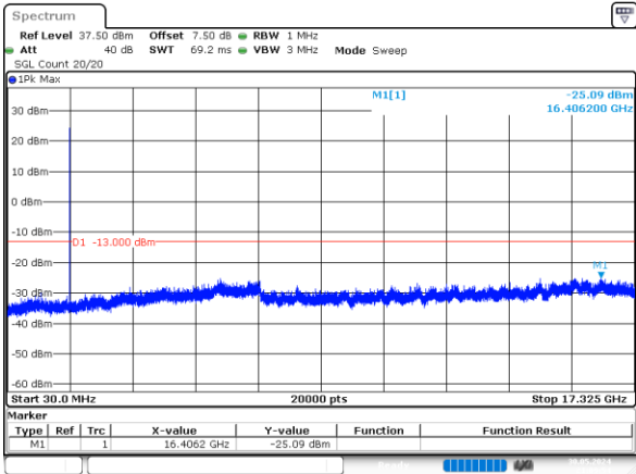
1.4MHz_Middle_QPSK_1@0 -25.09dBm
