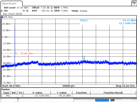
10MHz_High_QPSK_50@0 -34.15dBm
