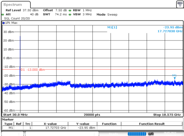
15MHz_Low_QPSK_1@0 -23.95dBm
