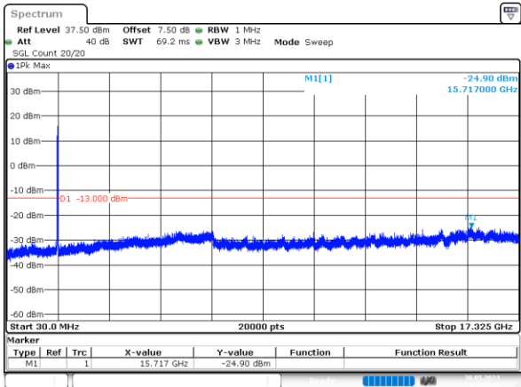
15MHz_Middle_QPSK_75@0 -24.90dBm
