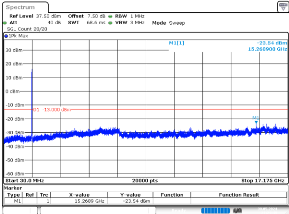
15MHz_Low_QPSK_75@0 -23.54dBm
