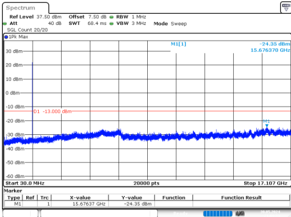
1.4MHz_Low_QPSK_6@0 -24.35dBm
