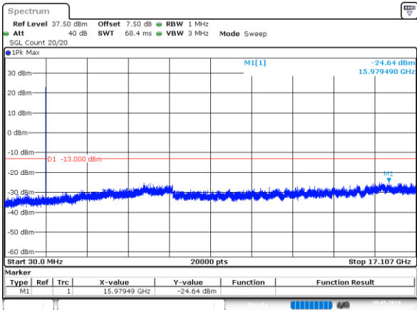
1.4MHz_Low_QPSK_1@0 -24.64dBm
