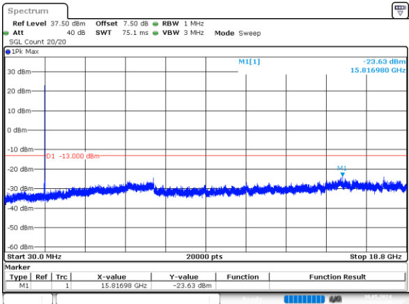
15MHz_Middle_QPSK_1@0 -23.63dBm
