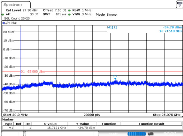
15MHz_Low_QPSK_1@0 -34.78dBm
