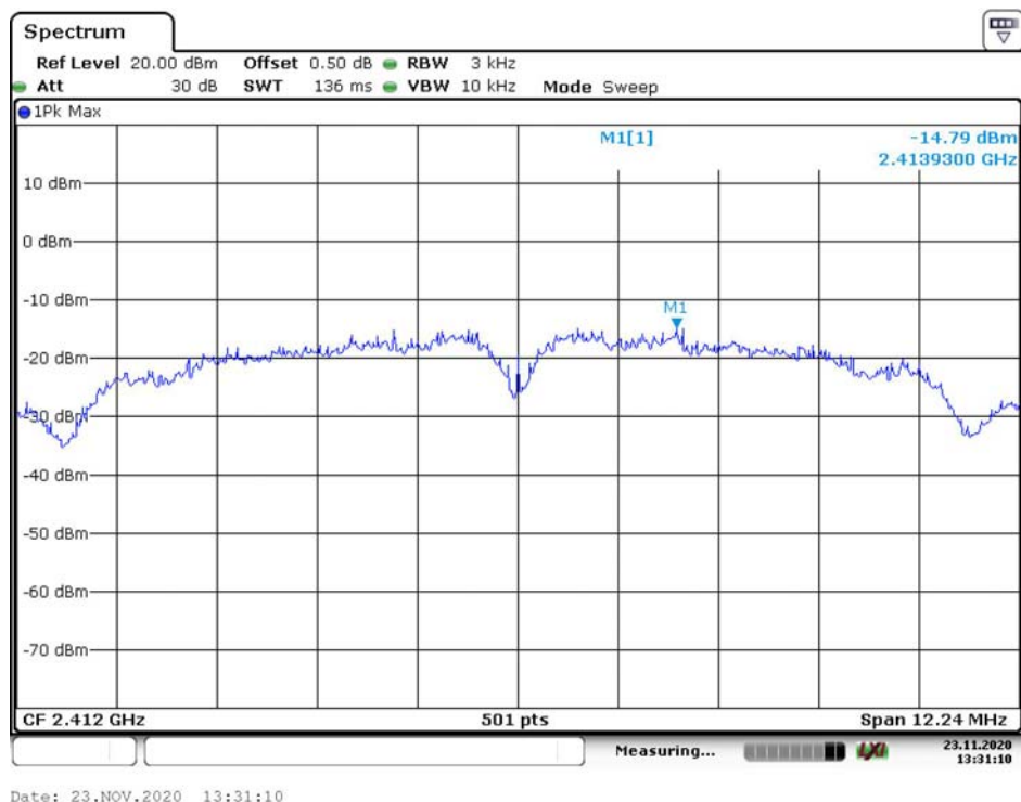
Power Spectral Density, 802.11b Low Channel
