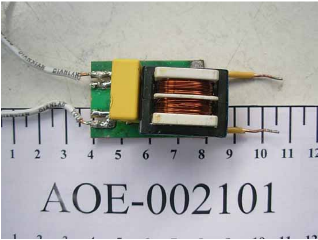
FIGURE 15 FLUORESCENT LUMINAIRES (M/N: TOP-10W) MAIN BOARD (COMPONENT SIDE)
