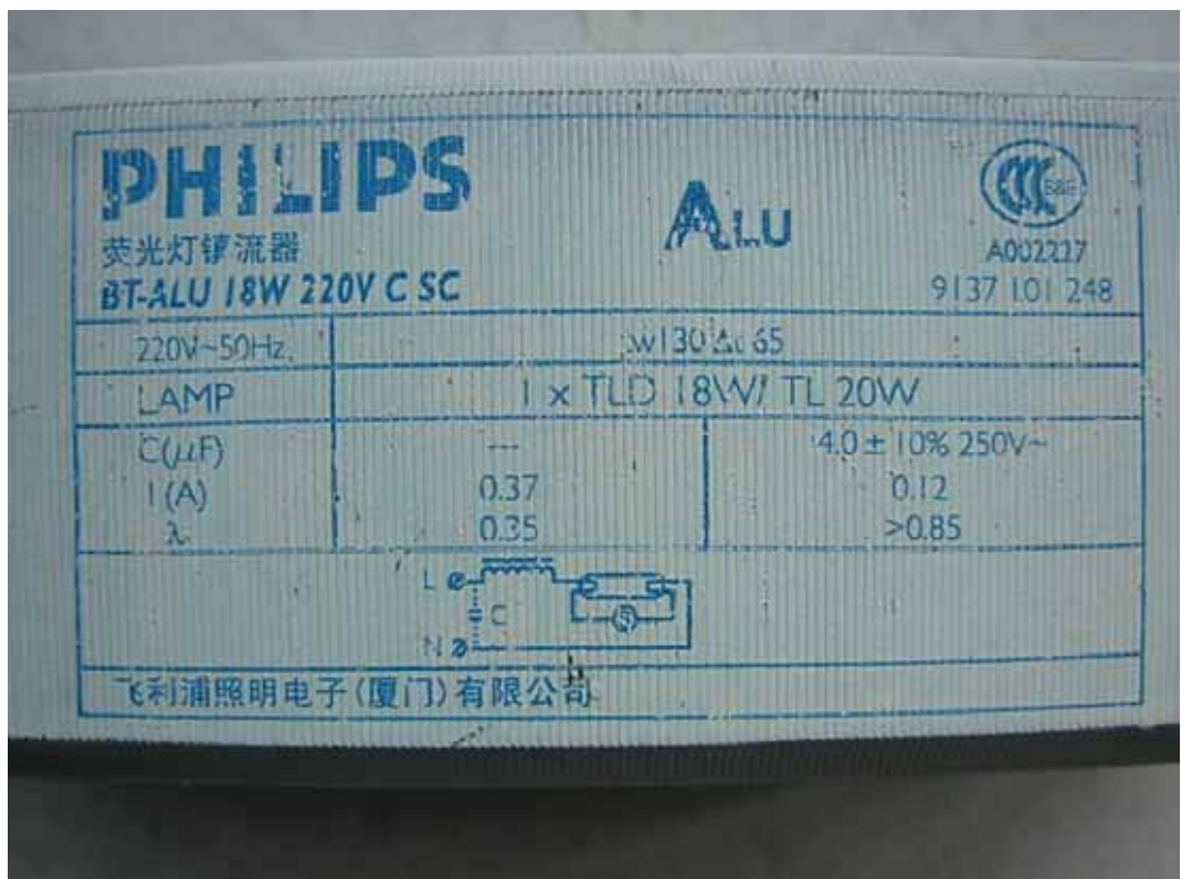
FIGURE 18 FLUORESCENT LUMINAIRES (M/N: TOP-10W) LABEL ON BALLAST
