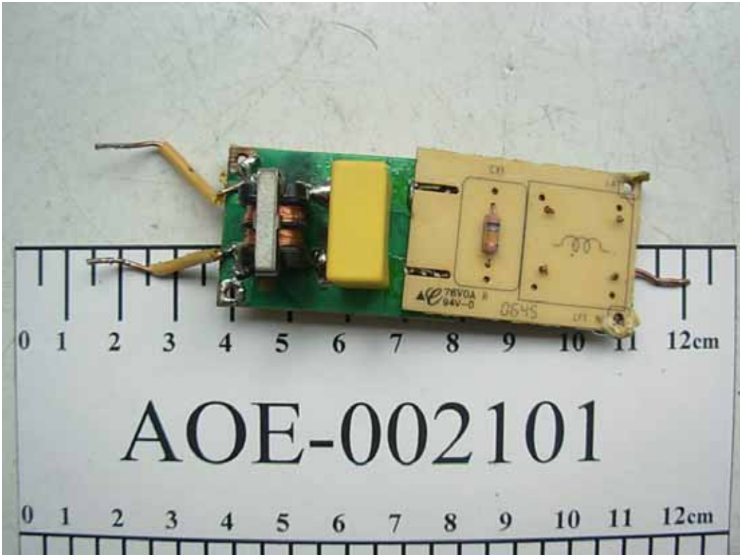
FIGURE 2 FLUORESCENT LUMINAIRES (M/N: TOP-20W) MAIN BOARD (COMPONENT SIDE)
