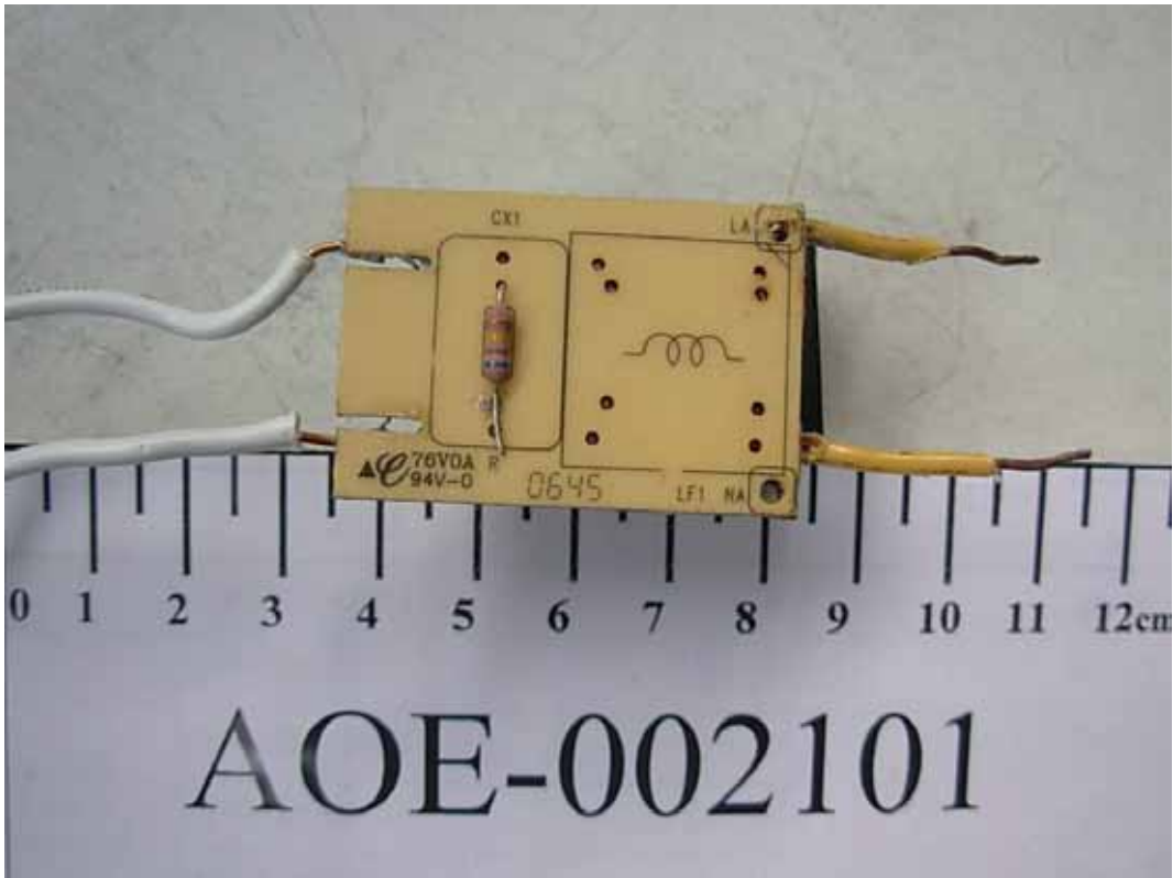
FIGURE 16 FLUORESCENT LUMINAIRES (M/N: TOP-10W) MAIN BOARD (SOLDERED SIDE)
