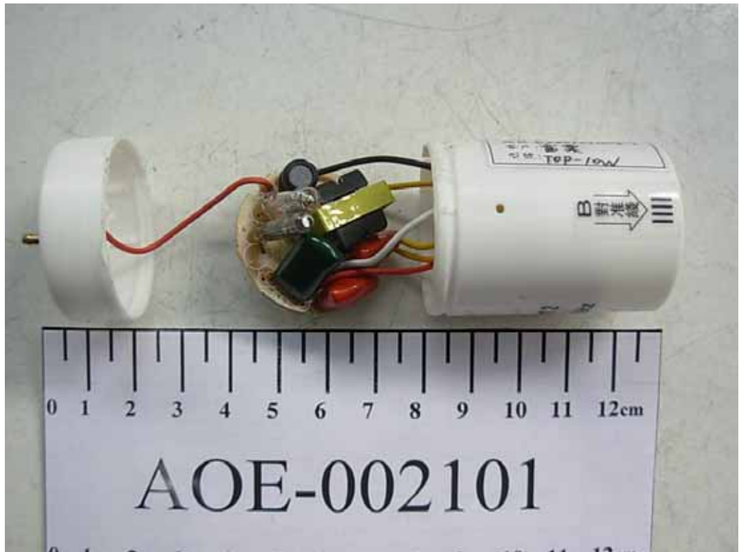
FIGURE 21 FLUORESCENT LUMINAIRES (M/N: TOP-10W) COVER REMOVED OF HEAD 1
