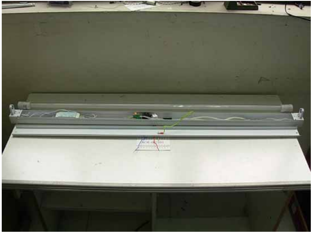
FIGURE 1 FLUORESCENT LUMINAIRES (M/N: TOP-20W) COVER REMOVED
