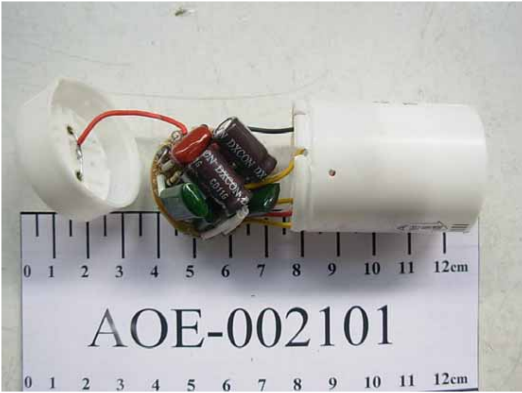
FIGURE 24 FLUORESCENT LUMINAIRES (M/N: TOP-10W) COVER REMOVE OF HEAD 2
