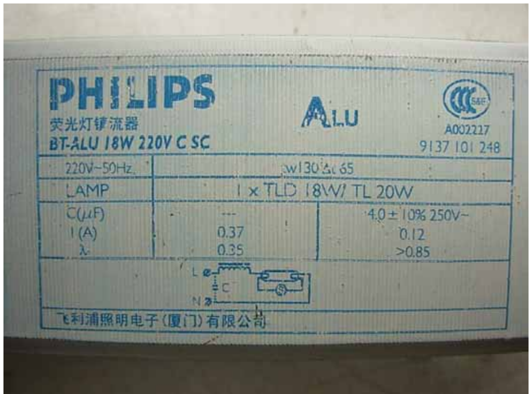
FIGURE 5 FLUORESCENT LUMINAIRES (M/N: TOP-20W) LABEL ON BALLAST
