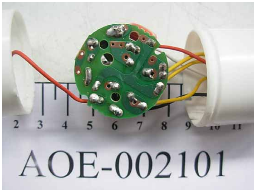
FIGURE 23 FLUORESCENT LUMINAIRES (M/N: TOP-10W) HEAD 1 MAIN BOARD (SOLDERED SIDE)
