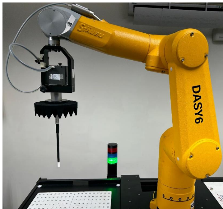
Fig.1 Photograph of the mmW measurement system
