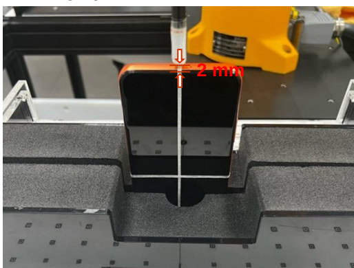
Photograph 3. PD, Back Surface, 2mm
