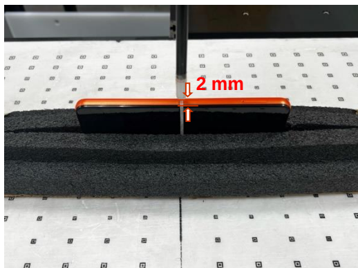
Photograph 7. PD, Right Edge, 2mm
