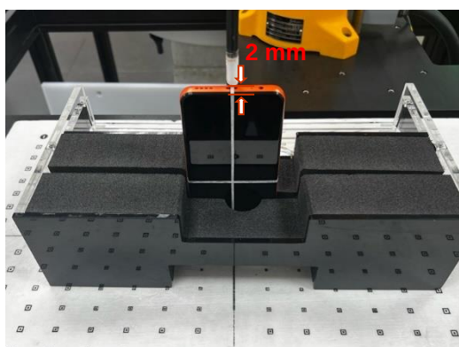
Photograph 11. PD, Bottom Edge, 2mm
