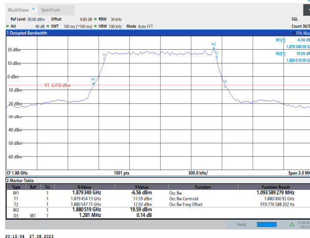
Band2-1.4MHz-16QAM-18900-6RB#0
