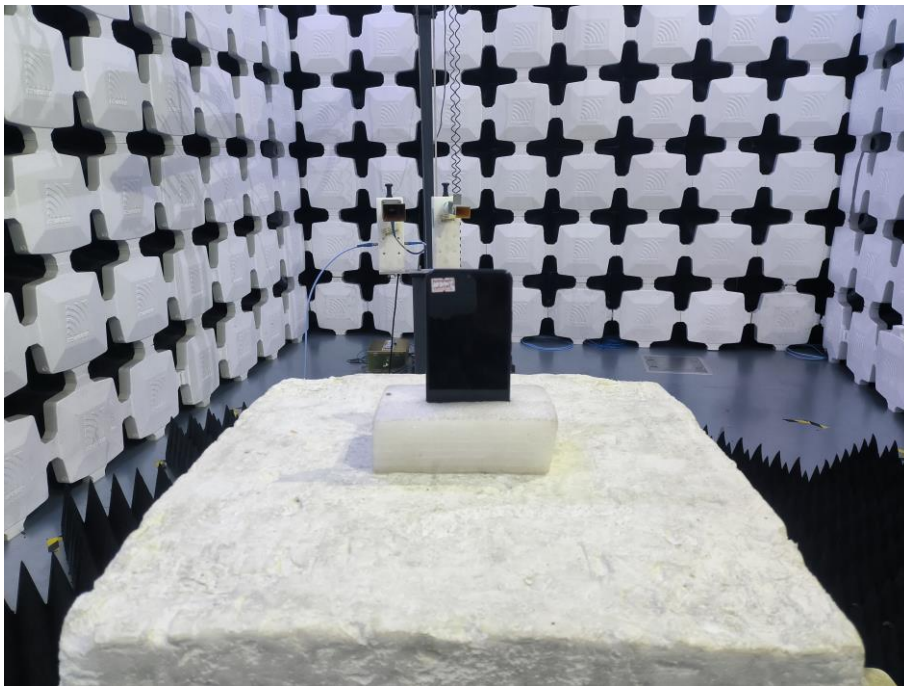
10. Radiated Emissions (Part 15C Wi-Fi/Bluetooth, 18GHz -26.5GHz)
