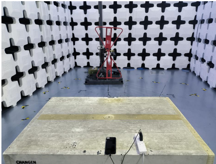
4. Radiated Emissions (Part 15B Camera/Video Player/WCDMA receiver/LTE receiver, 30MHz-1GHz)
