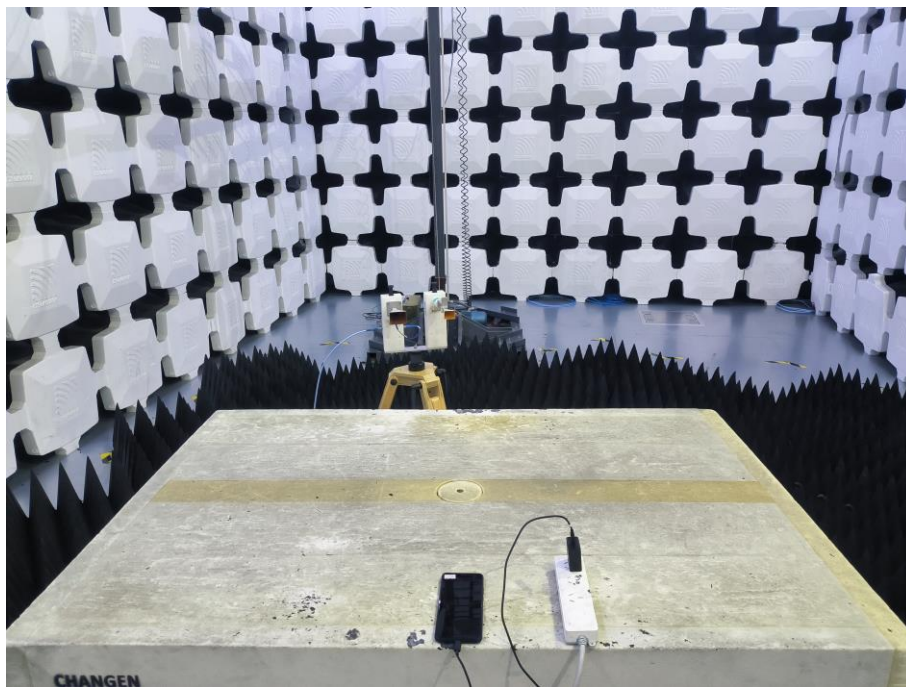
6. Radiated Emissions (Part 15B Camera/Video Player/WCDMA receiver/LTE receiver, 18GHz-26.5GHz)
