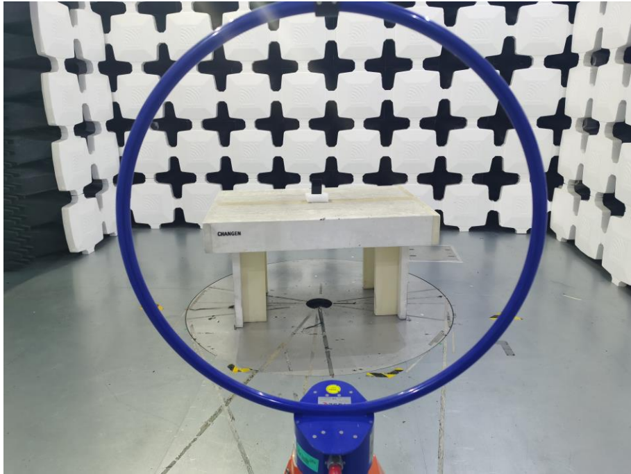
7. Radiated Emissions (Part 15C Wi-Fi/Bluetooth/NFC, 9kHz-30MHz)
