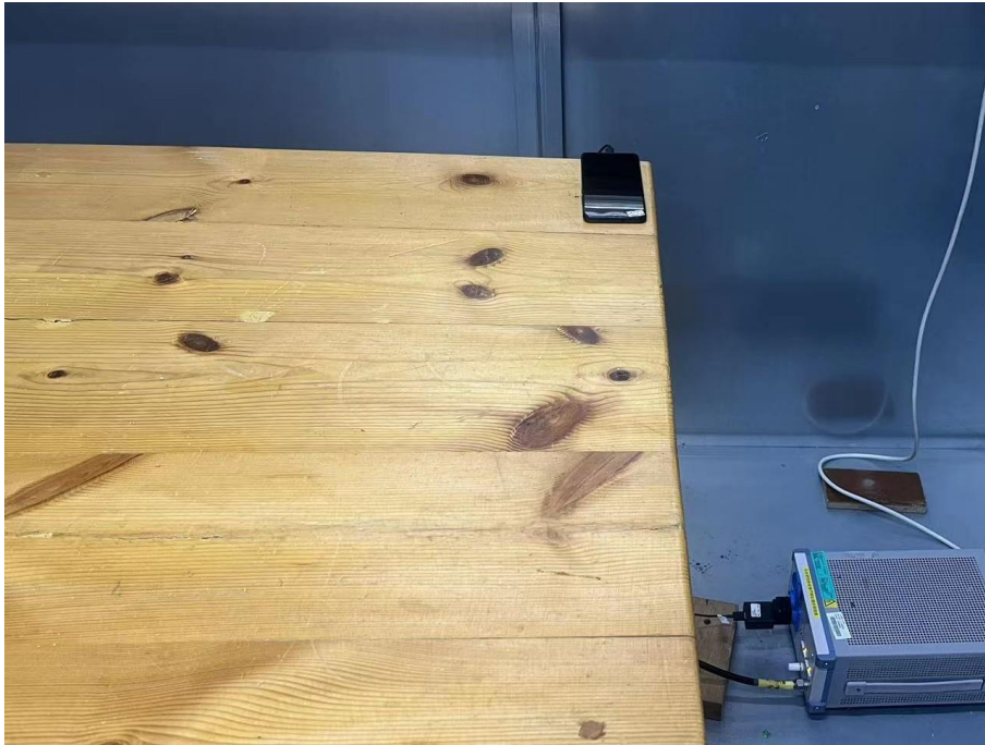
15. Conducted Emission (Part 15B, Camera/Video Player)
