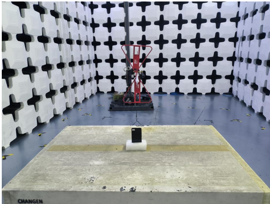
8. Radiated Emissions (Part 15C Wi-Fi/Bluetooth/NFC, 30MHz-1GHz)
