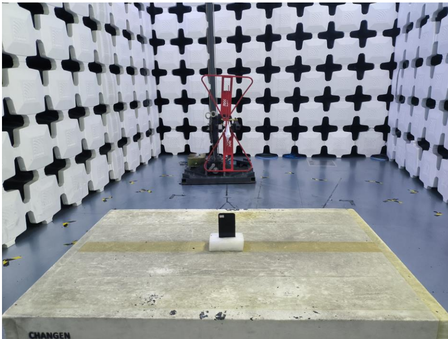
12. Radiated Emissions (Part 22/24/27,30MHz-1GHz)
