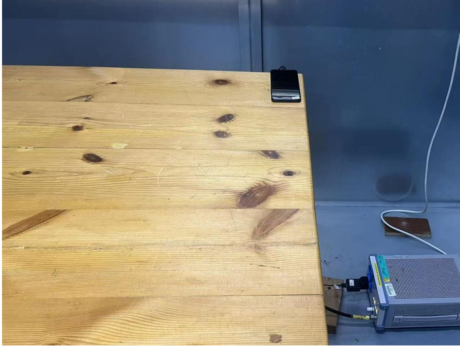
17. Conducted Emission (Part 15C, Wi-Fi/Bluetooth)
