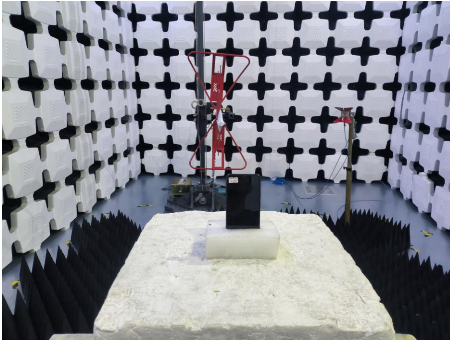
9. Radiated Emissions (Part 15C Wi-Fi/Bluetooth, 1GHz -18GHz)
