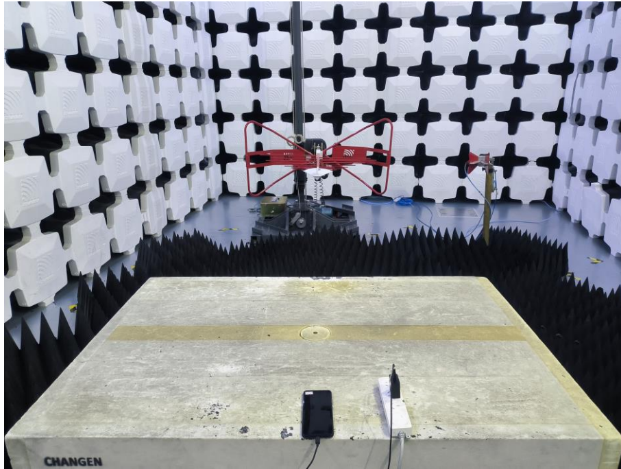
5. Radiated Emissions (Part 15B Camera/Video Player/WCDMA receiver/LTE receiver,1GHz-18GHz)
