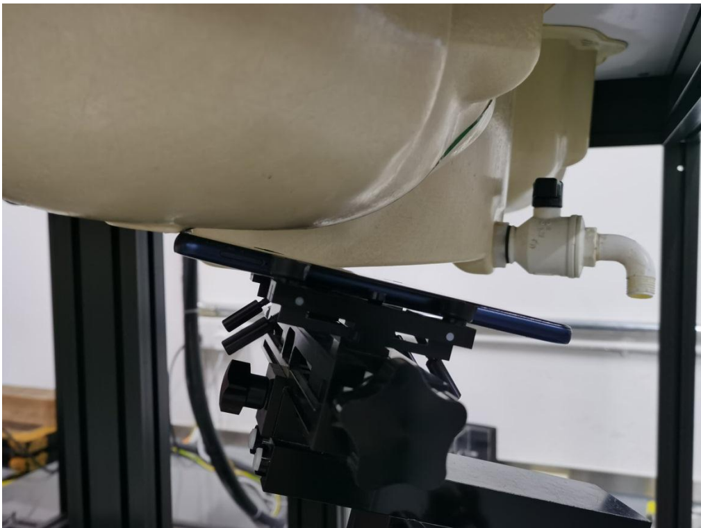
Picture 8: Right Tilt 15° Position
