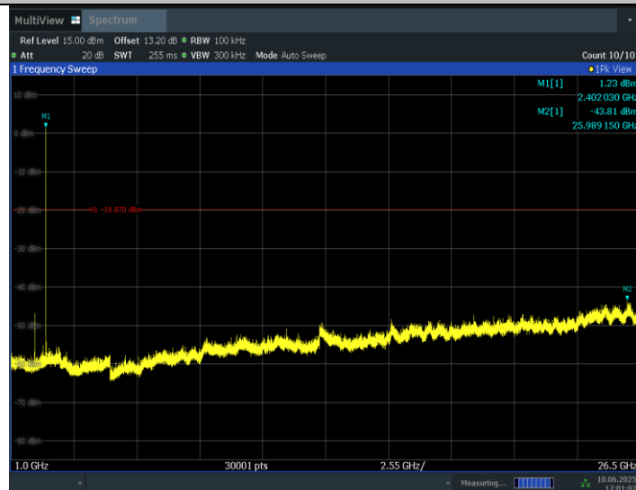
BLE_1M_Ant5_2402_1000~26500
