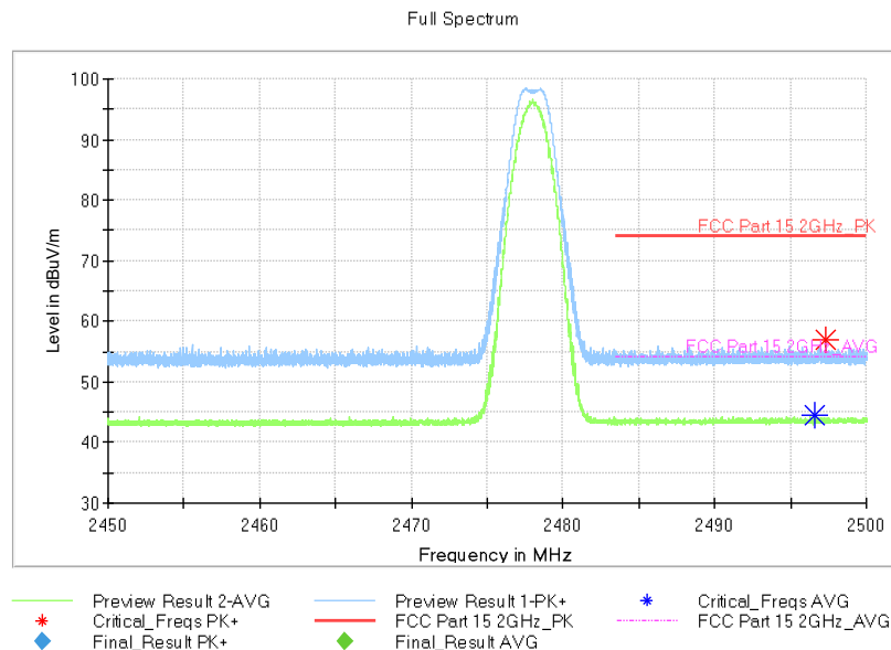
Fig.2. Frequency Band Edges: GFSK, 2478 MHz, Hopping Off, 2.45 GHz - 2.50GHz
