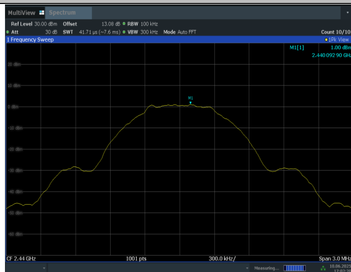
BLE_1M_Ant5_2440_0~Reference
