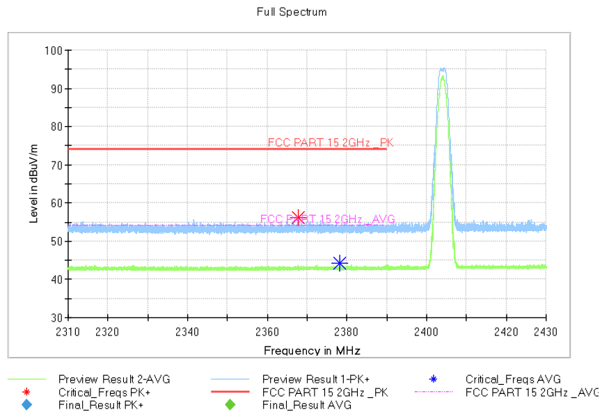
Fig.1. Frequency Band Edges: GFSK, 2404 MHz, Hopping Off, 2.31 GHz – 2.43GHz
