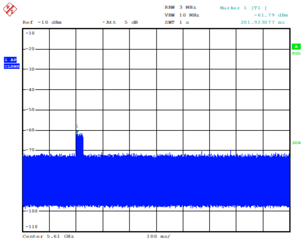
Fig.A.1 80M Calibration Result
