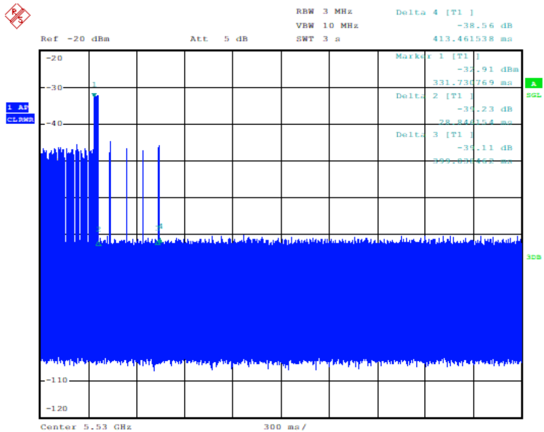
Fig.A.5 channel closing transmission time
