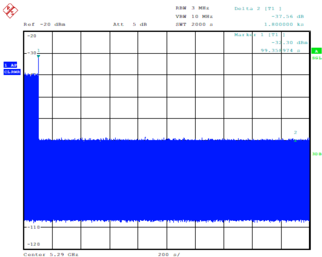
Fig.A.6 Non-Occupancy Period
