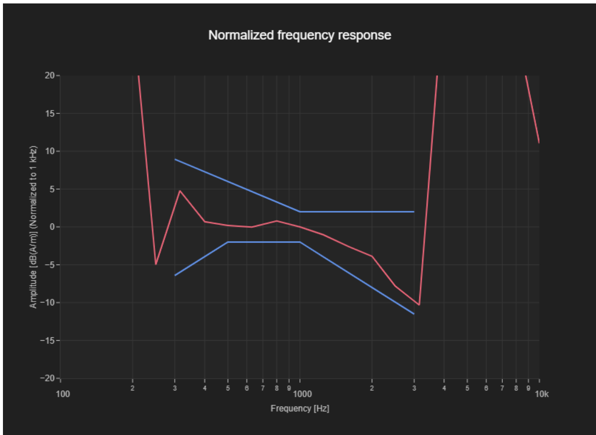
Figure C.2 Frequency Response of NR B30-N77-OTT
