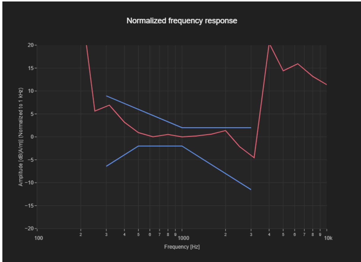
Figure C.1 Frequency Response of NR B2-N77
