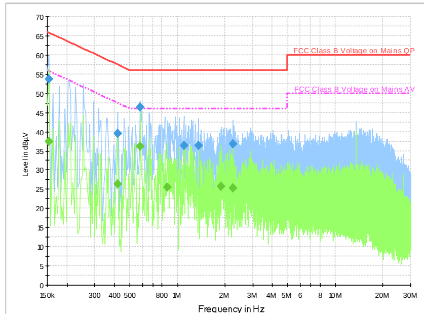
Figure B-11: Measurement results for Conducted Emission
