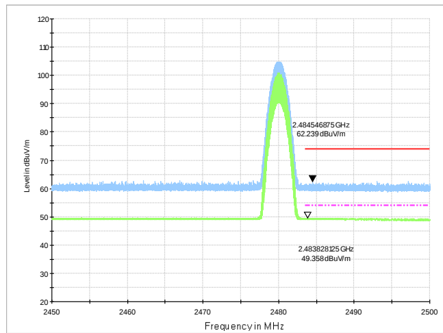
Fig.63. Frequency Band Edges: 8DPSK, Channel 78, 2.45 GHz - 2.50GHz
