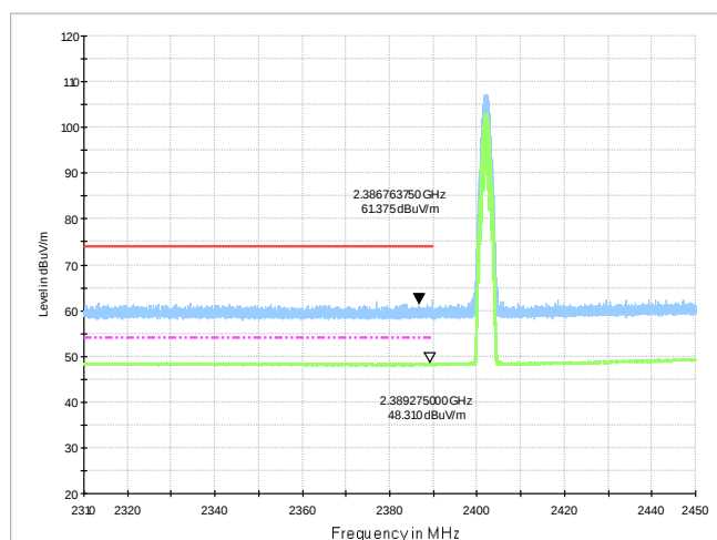
Fig.62. Frequency Band Edges: 8DPSK, Channel 0, 2.31 GHz - 2.45GHz
