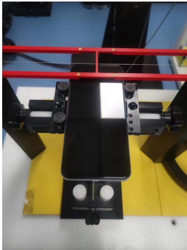
Picture 2: EUT Positioning for RF/T-coil
