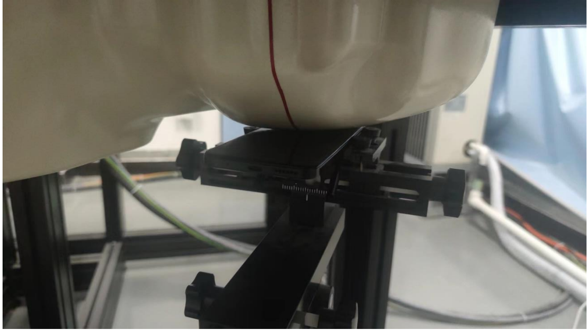
Picture 2: Left Head Touch Cheek Position
