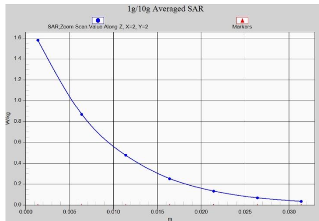
Fig. 1-22 Z-Scan at power reference point (LTE Band30 Body)
