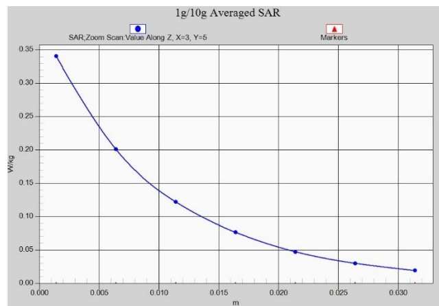
Fig. 1-21 Z-Scan at power reference point (LTE Band30 Head)
