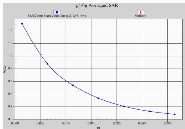
Fig. 1-14 Z-Scan at power reference point (LTE Band 4 Body)
