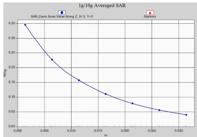
Fig. 1-13 Z-Scan at power reference point (LTE Band 4 Head)
