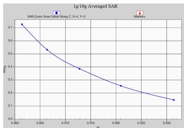
Fig. 1-20 Z-Scan at power reference point (LTE Band14 Body)
