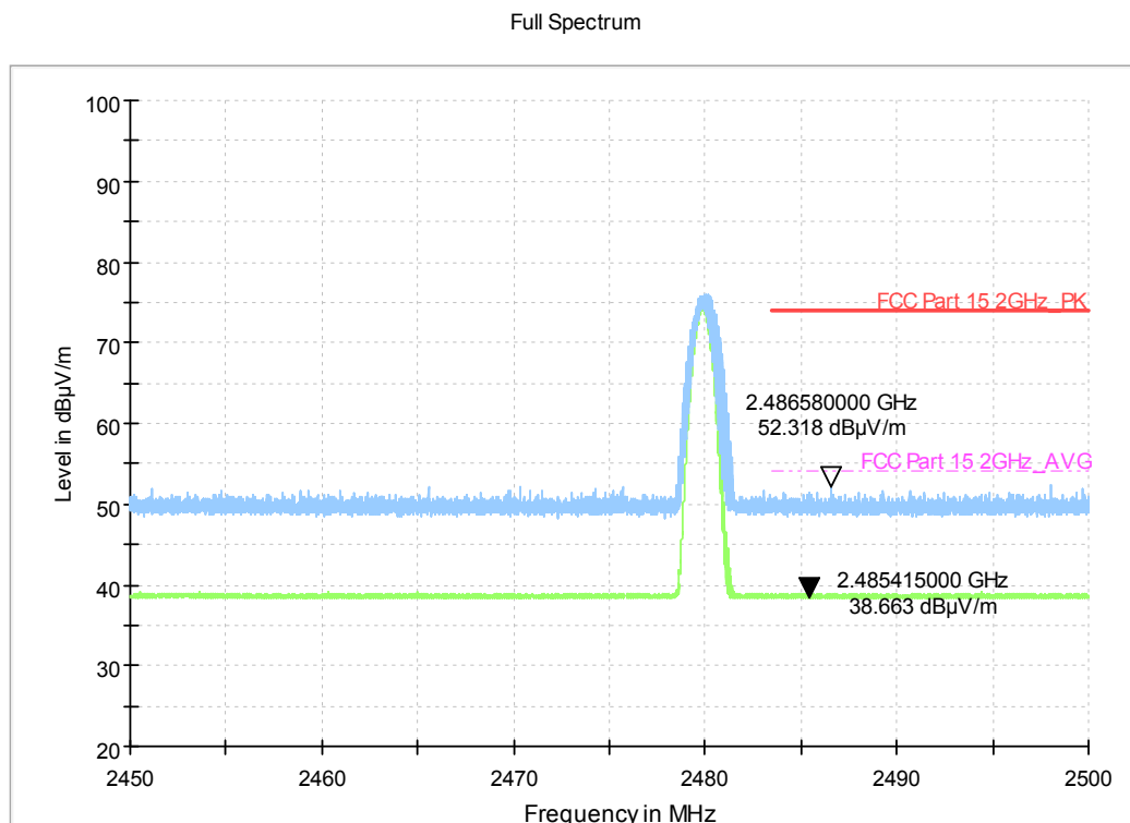
Fig.61. Radiated emission (Power): \pi/4 DQPSK, high channel
