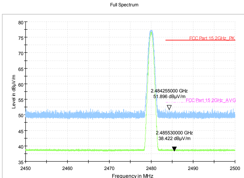
Fig.59. Radiated emission (Power) GFSK, high channel
