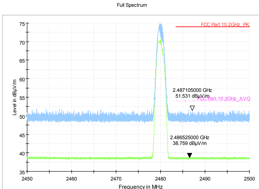
Fig.63. Radiated emission (Power): 8DPSK, high channel
