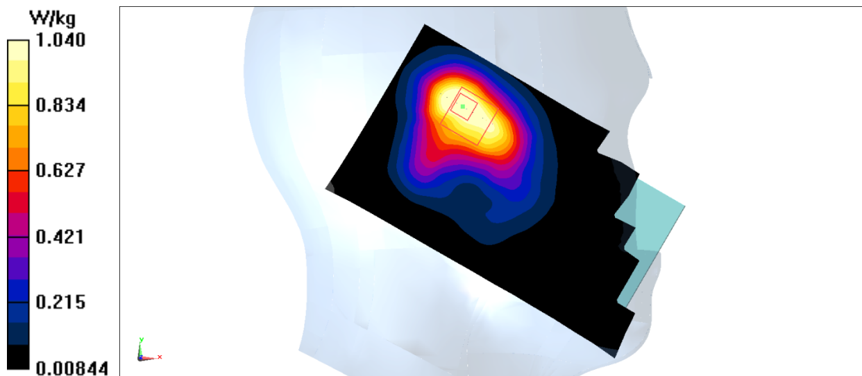
Fig.29 2450 MHz
