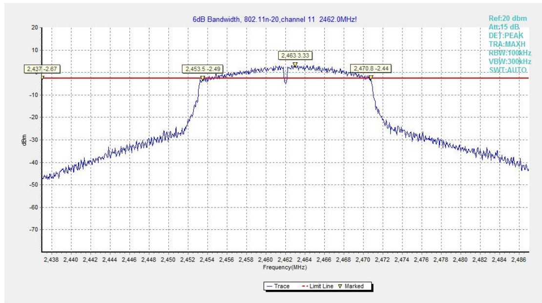
Fig.A.4.9 Occupied 6dB Bandwidth (802.11n-HT20, Ch 11)
