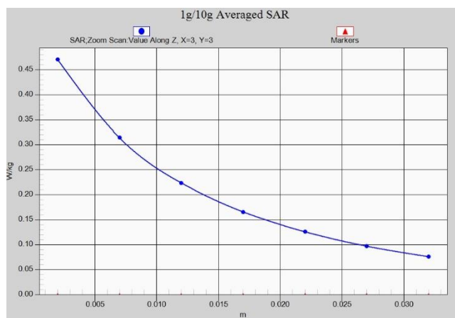
Fig. 1-15 Z-Scan at power reference point (LTE Band14)
