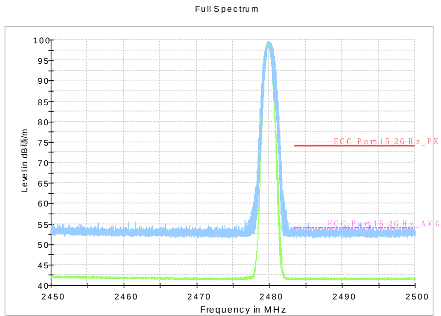
Fig.16. Frequency Band Edges: \pi/4 DQPSK, Channel 78, 2.45 GHz - 2.50
