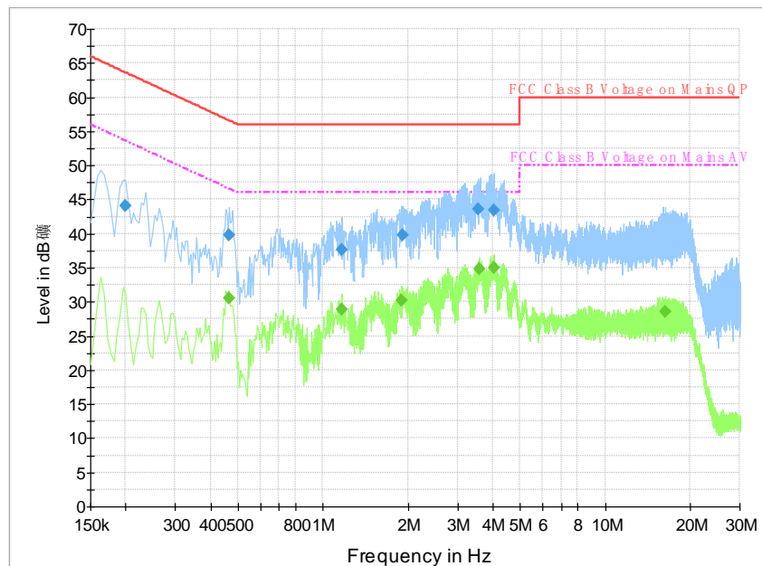
Fig.A.9.3 AC Powerline Conducted Emission-Traffic(with AE3)
