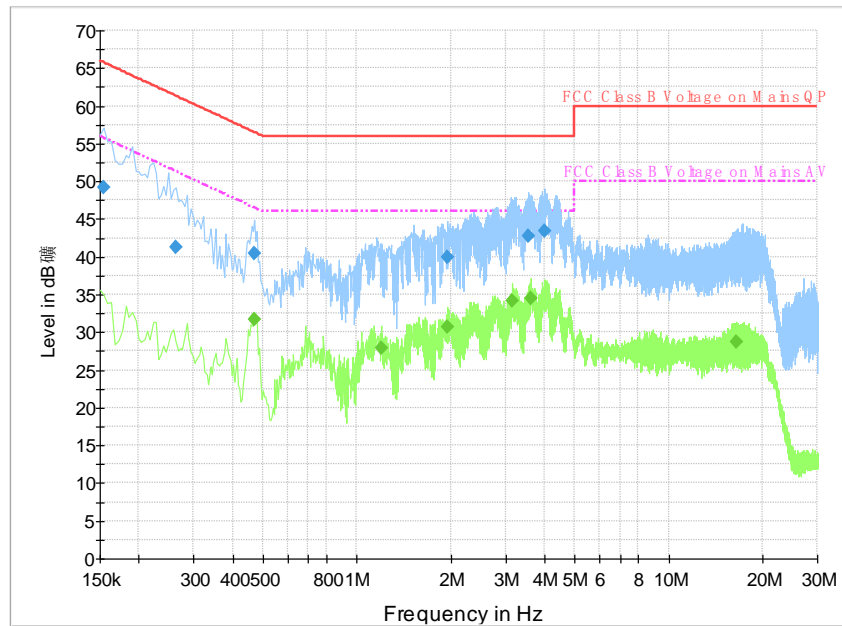
Fig.A.9.2 AC Powerline Conducted Emission-Traffic(with AE2)
