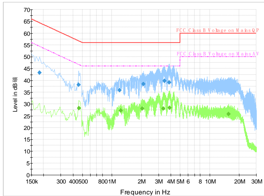
Fig.A.9.4 AC Powerline Conducted Emission-Idle(with AE3)
