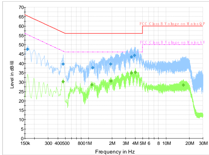
Fig.A.9.1 AC Powerline Conducted Emission-Traffic(with AE2)
