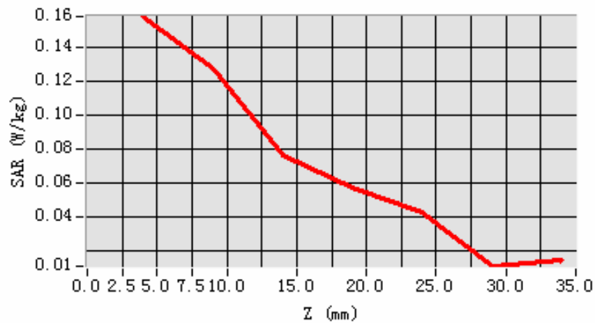
SAR, Z Axis Scan (X = -8, Y = -36)
