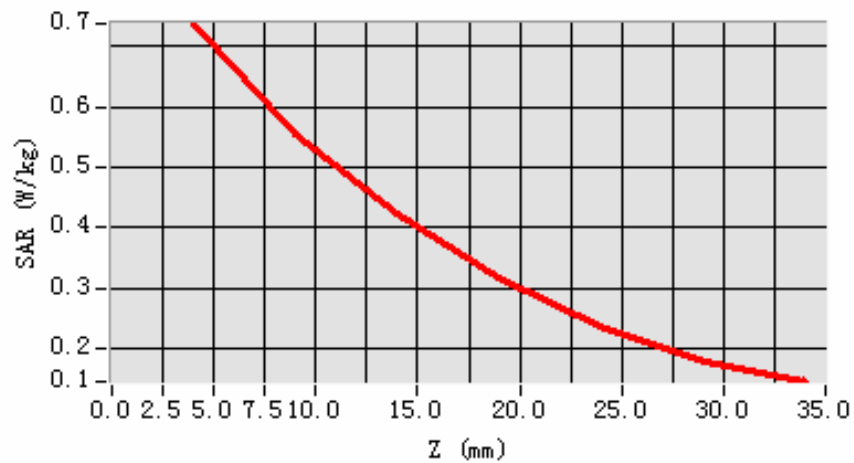
SAR, Z Axis Scan (X = -33, Y = -24)
