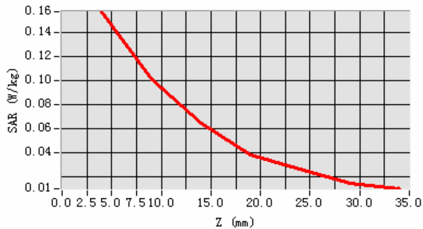
SAR, Z Axis Scan (X = 11, Y = 15)
