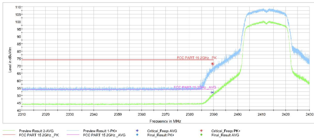
Fig.5 Transmitter Spurious Emission - Radiated (Power): 802.11n-HT20, ch1, 2.31 GHz - 2.43GHz
