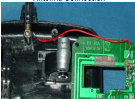
Antenna Connection
