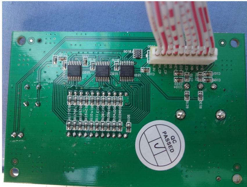
Panel Back View
