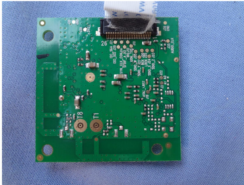
RF PCB Back View
