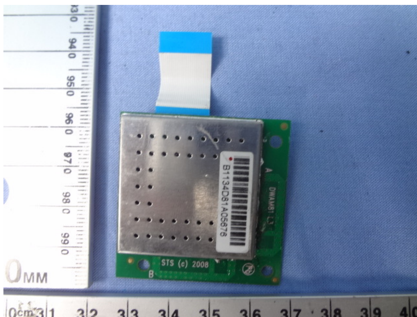
RF PCB Front View
