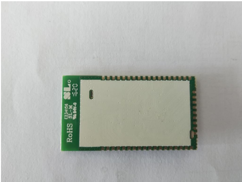
(2) EUT Photo (M/N: HSBT3007-EA)
