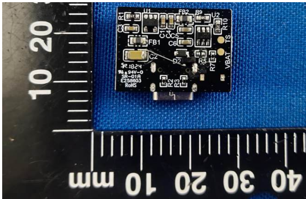
SECONDARY BOARD 2 TOP VIEW
