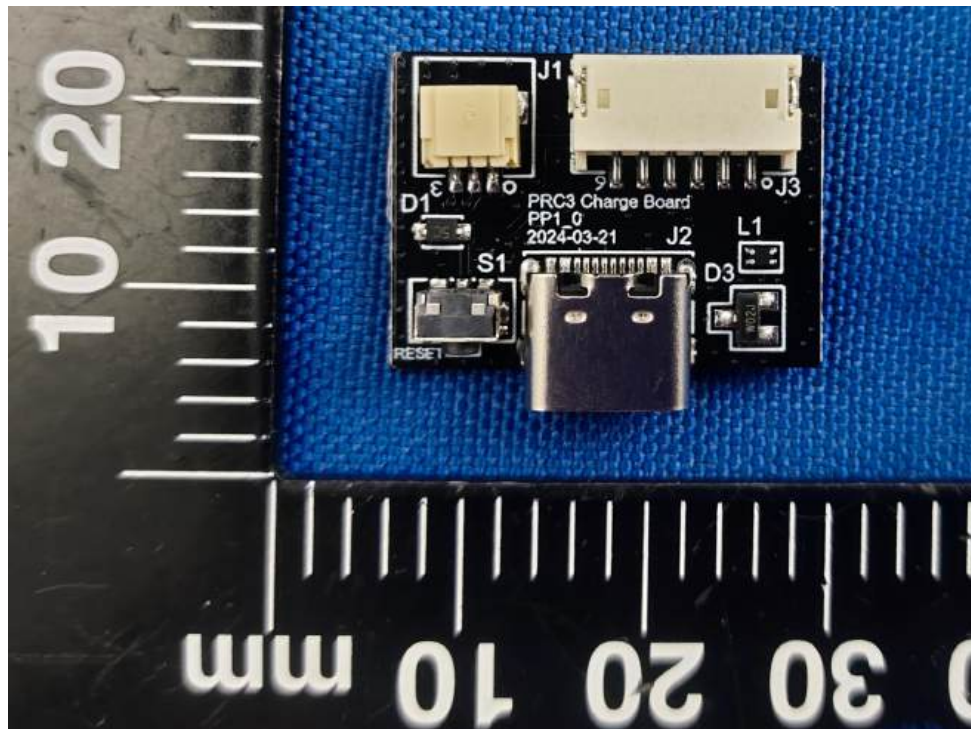
SECONDARY BOARD 1 TOP VIEW
