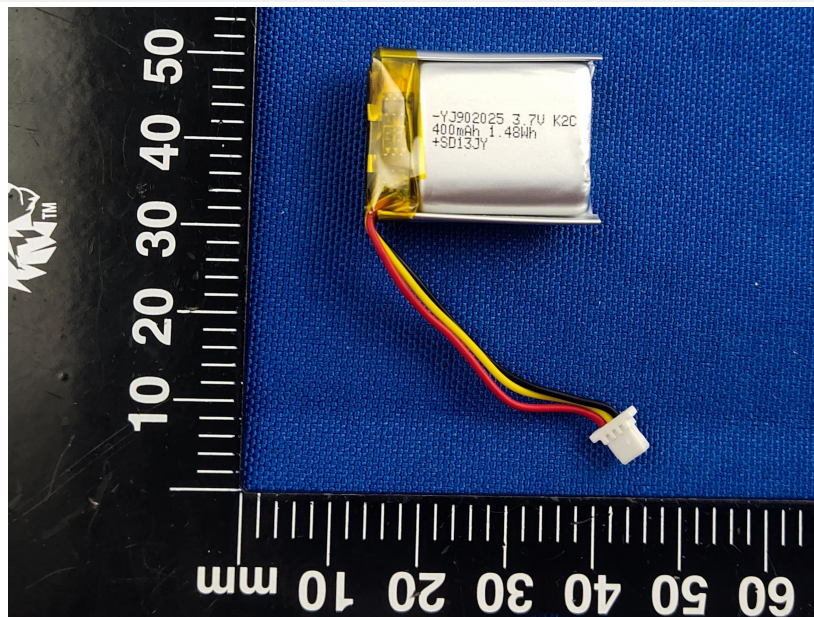
BATTERY(FRONT)
